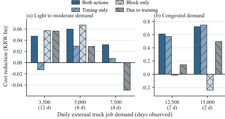
Fig. 5: Cost reduction by demand level, decomposed by action range; the values are those of Table 3. The vertical axis is split by demand because the two congested levels are more than ten times larger than the rest: (a) 3,500–7,500 and (b) 12,500–15,000 trucks per day, with the number of days observed printed under each tick. The first three bars are measured against no reallocation. The fourth bar, set slightly apart, uses a different baseline: it is the trained model minus the untrained one, that is, the last column of Table 3. Arrival-time adjustment carries 91.3% of the total reduction, whereas block-only reallocation turns negative once demand is congested.
