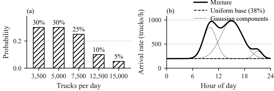
Fig. 3: External truck job demand. (a) The five daily demand levels and the probability with which each is drawn, independently for each day. (b) The time-of-day arrival process at 12,500 trucks per day, with the uniform base and the three Gaussian components drawn separately beneath the mixture they sum to. The literature supports the demand magnitudes and the fact that arrivals are far from uniform over the day, whereas the shape of the mixture is a construction of this study.
