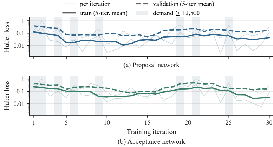
Fig. 3: Training and validation loss over the 30 iterations; the faint line is the per-iteration value beneath a five-iteration mean, and the vertical axis is logarithmic. Shading marks the iterations whose demand level was 12,500 or above, so much of the visible fluctuation follows that draw rather than the fit. Exploration fell linearly from 0.50 to 0.05.
