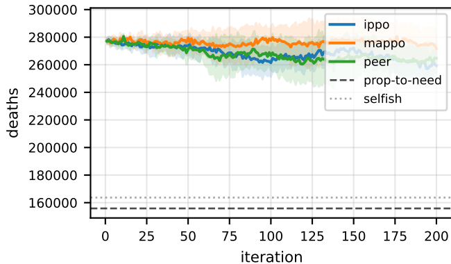
Total deaths (lower=better)
