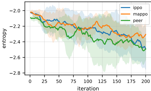
Policy entropy (higher=more random)
