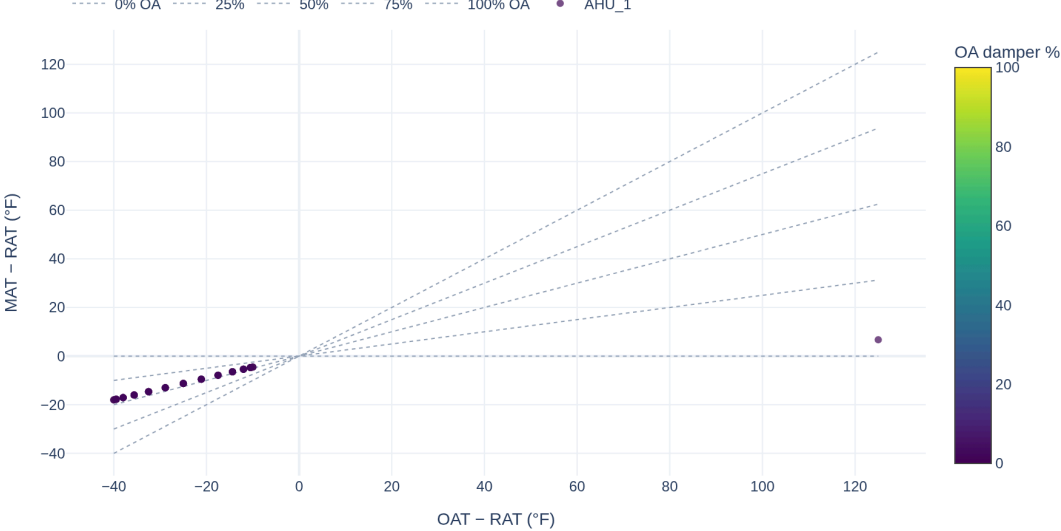
Economizer free-cooling delta scatter (fan on, |OAT - RAT| \geq 10^\circ F )
