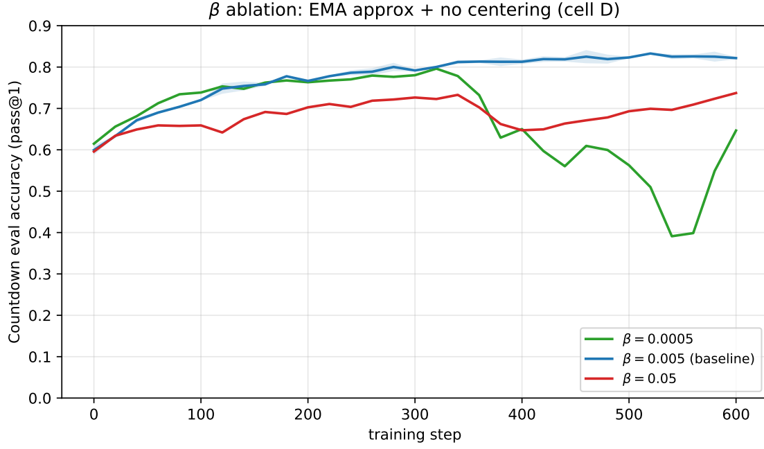
FIGURE 11. \beta ablation on no-centering approx KL (cell D). Baseline \beta = 0.005 vs. \beta = 0.05 ( 10\times ) and \beta = 0.0005 ( 0.1\times ). The cell is robust to weakening \beta (no early-run impact at \beta = 0.0005 ) but slower learning at \beta = 0.05 .
