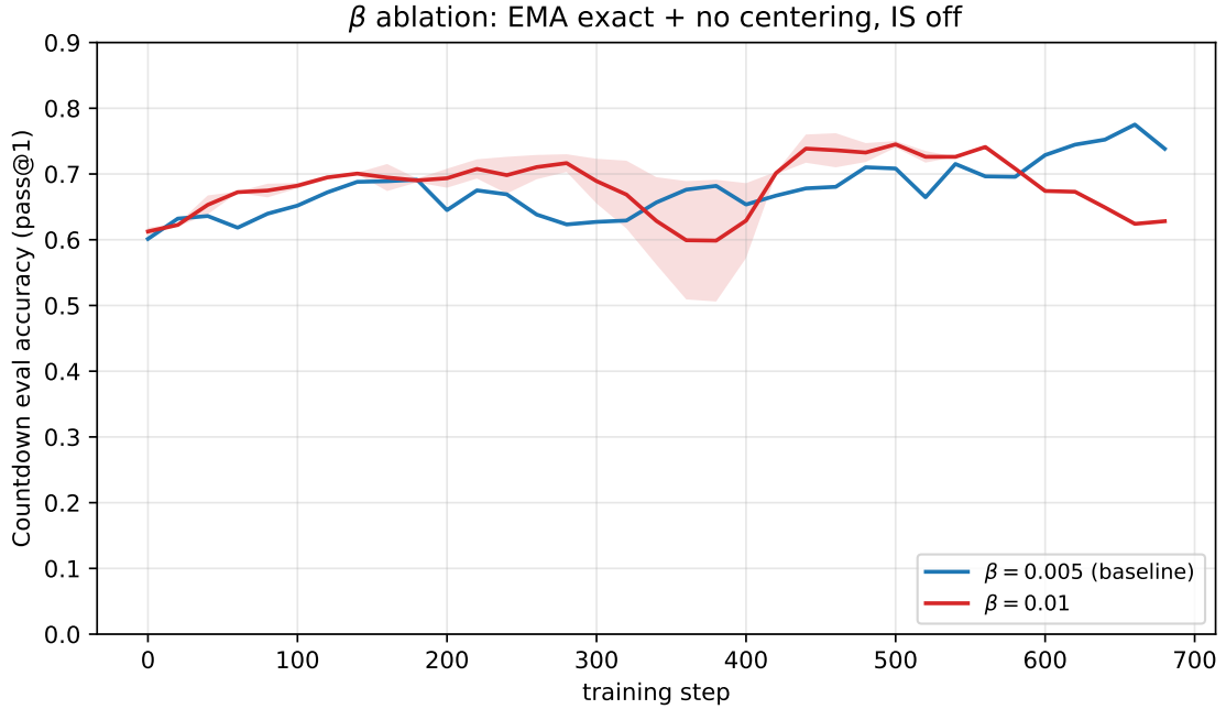
FIGURE 8. \beta ablation on no-centering exact KL with IS off (B-noIS family).
