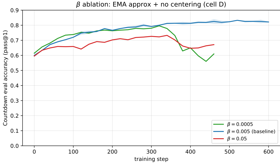
FIGURE 10. \beta ablation on no-centering approx KL (cell D). Baseline \beta = 0.005 vs. \beta = 0.05 ( 10\times ) and \beta = 0.0005 ( 0.1\times ). The cell is robust to weakening \beta (no early-run impact at \beta = 0.0005 ) but slower learning at \beta = 0.05 .
