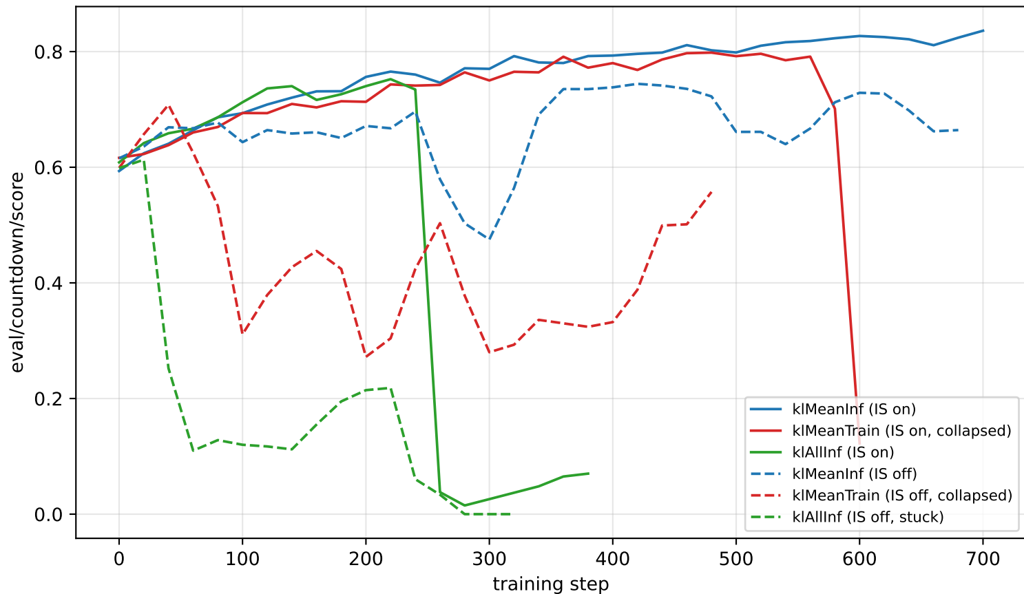
Reset-reference baseline (no EMA): KL-source \times IS
