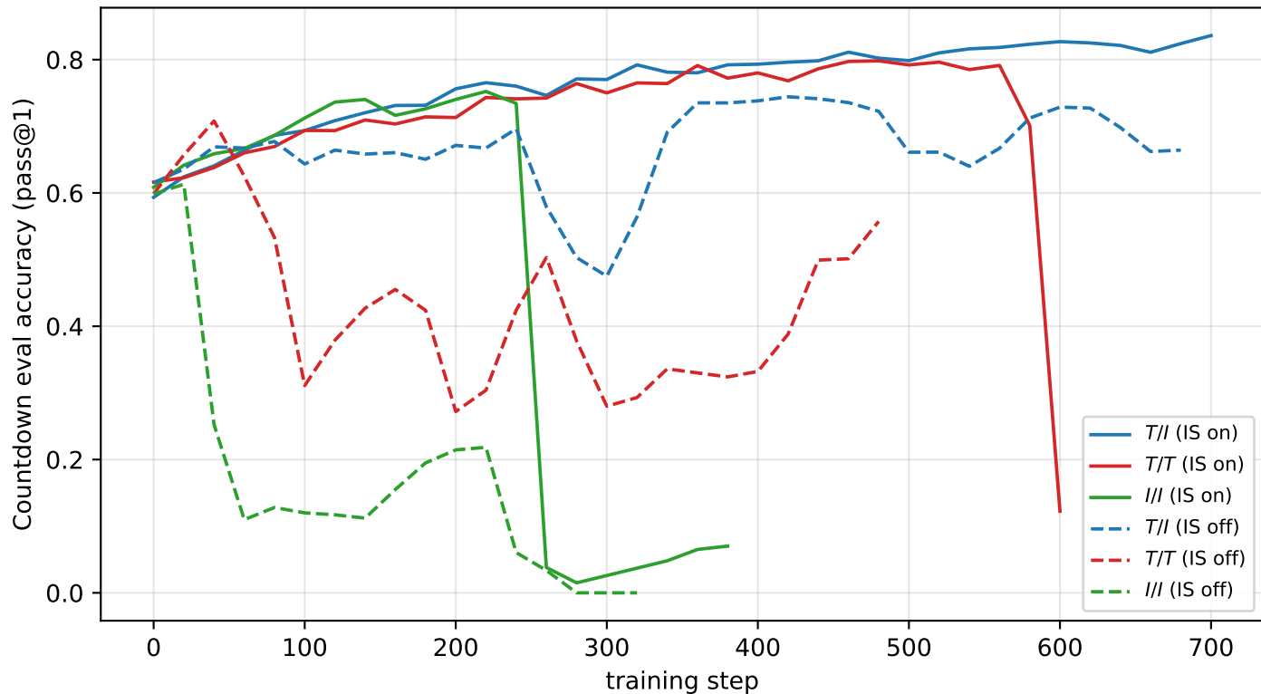
Periodic-reset reference (every 50 steps): KL-source \times IS
