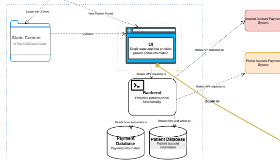
C2: CONTAINER DIAGRAM
