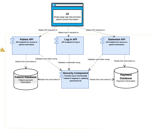
C3: COMPONENTS DIAGRAM
