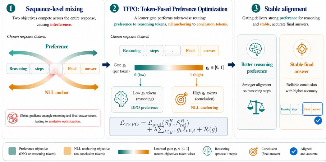
Figure 2: Overview of TFPO. A learned gate routes response tokens between preference shaping and likelihood anchoring, targeting reasoning-sensitive and answer-bearing regions, respectively. The displayed loss is schematic: routed DPO sequence scores are defined in Eqs. (2)–(4), and Eq. (9) gives the full objective.
