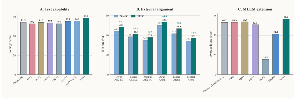
Figure 1: Summary of the main empirical picture. Left: TFPO achieves the best main ten-benchmark average among all compared methods, outperforming both SimPO and the NLL-anchored SimPO+NLL baseline on Qwen3-8B. Middle: TFPO consistently improves over SimPO on judge-based alignment benchmarks across Qwen, Llama, and Mistral backbones. Right: under multimodal preference tuning, TFPO yields the best average among the compared methods.
