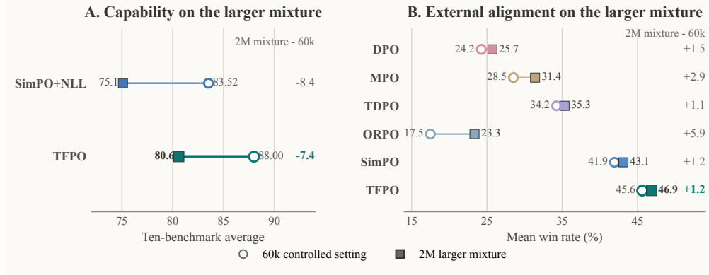
Figure 4: Robustness to a larger 2M preference mixture. Left: matched ten-benchmark averages for SimPO+NLL and TFPO in the controlled 60k setting and under the larger mixture. Right: external-alignment composites for the same settings, computed from AlpacaEval 2.0 LC/WR and Arena-Hard-v2.0-Preview WR across Qwen, Llama, and Mistral. Connecting lines compare the controlled 60k setting with the larger mixture, whose composition also differs.
