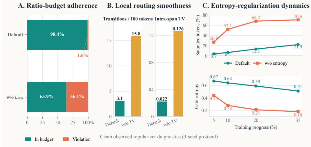
Figure 5: Regularizer-specific diagnostics. A: 98.4% of default responses satisfy the gate budget versus 63.9% without \mathcal{L}_{len} . B: removing TV increases transitions/100 tokens and intra-span TV from 3.1/0.022 to 15.8/0.126. C: without entropy regularization, 52.1% of tokens are saturated at 10% training progress, versus 6.4% by default.
