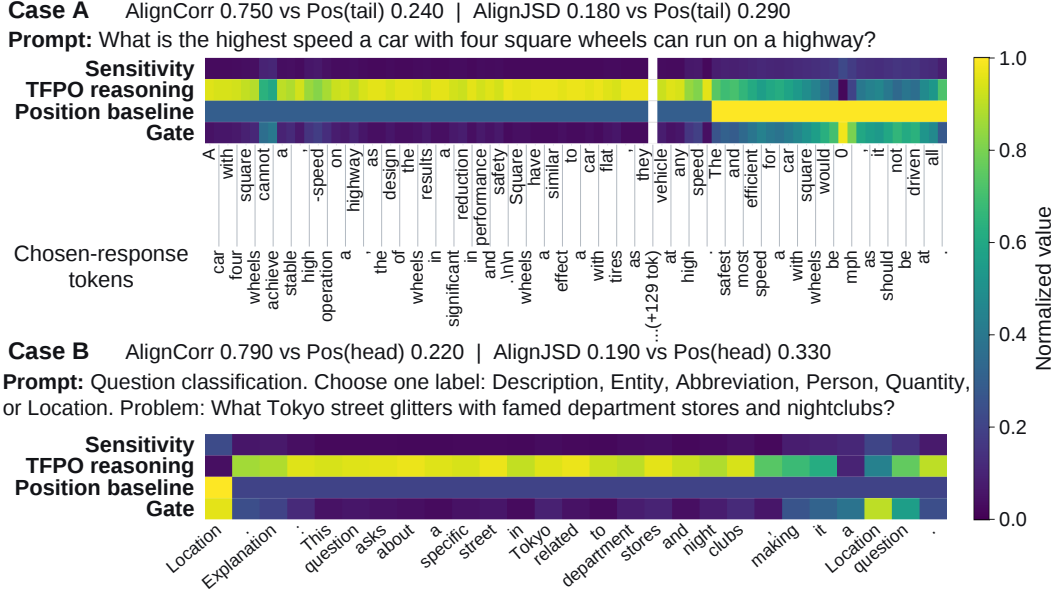
Figure 3: Held-out token-routing examples. Sensitivity denotes the normalized absolute policy-reference log-probability difference |\Delta \log p| . Other rows show TFPO reasoning weights, a matched-budget position baseline, and the gate. The gate highlights a final span in Case A and the answer-first label in Case B.
