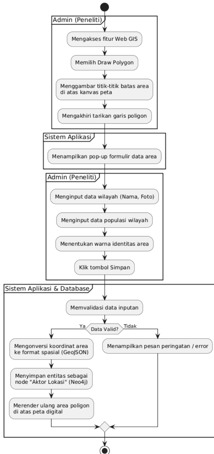
Gambar 3.4 Activity Diagram Pemetaan Area Kustom (Draw Poligon)
