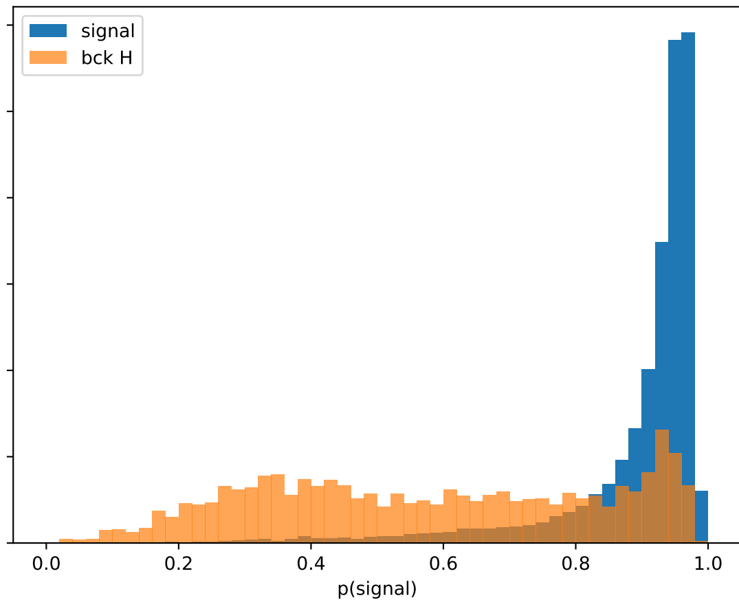
BDT(H) score
