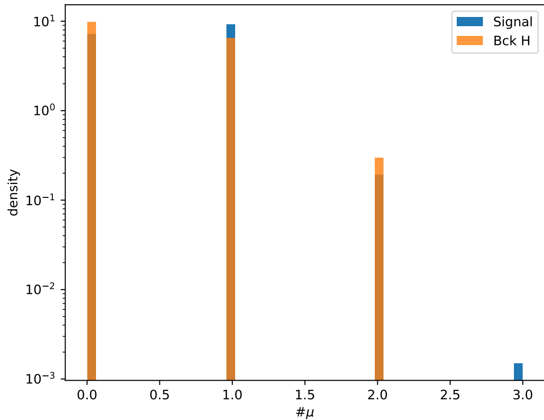
Isolated Muons
