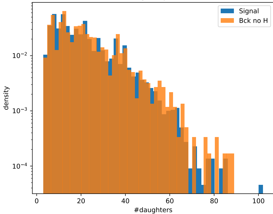
Daughter jet 1
