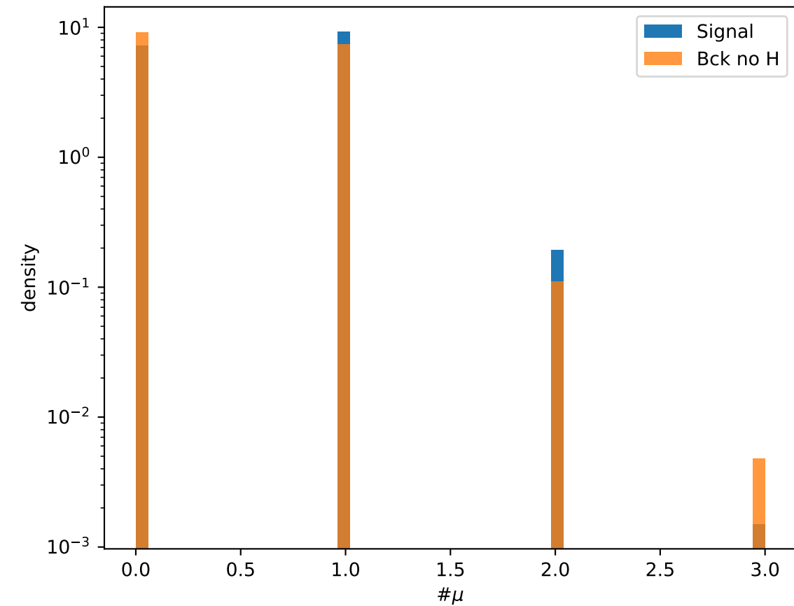
Isolated Muons
