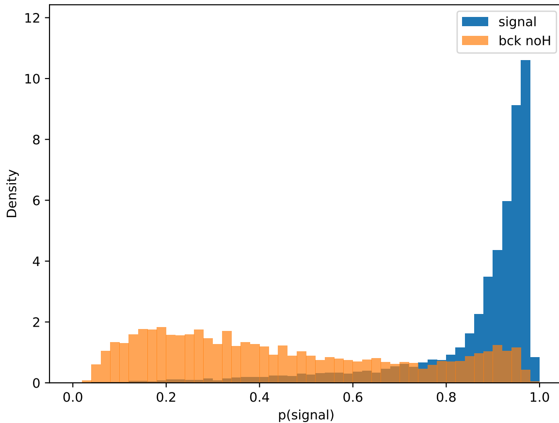
BDT(noH) score
