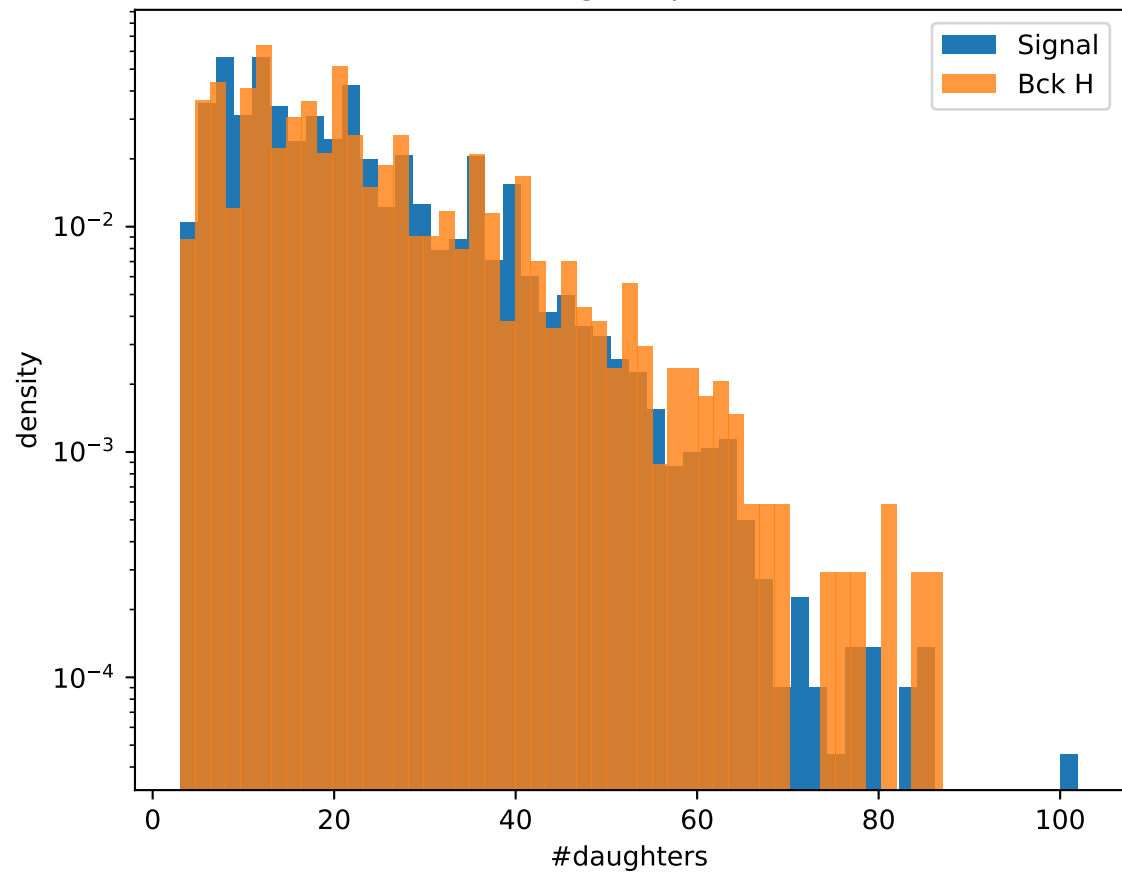
Daughter jet 1
