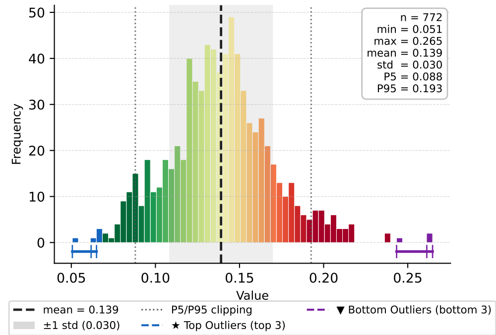
PDR (Lower is better)
