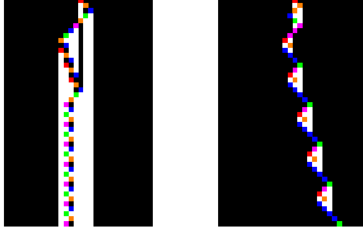
Figure 4: Space-time diagrams of the first 45 steps of a Cycler , 1RB---_ORCOLE_1LDOLA_1LB1RB_1LC1RC (left) and of the first 45 steps of a Translated Cycler , 1RB---_1LB1LC_ORDORC_1LE1RE_1LAOLE (right). Cyclers are machines that eventually repeat the same configuration forever. Translated Cyclers are machines that eventually repeat the same configuration forever, but translated in space. We refer to these two types of machines as loops .
