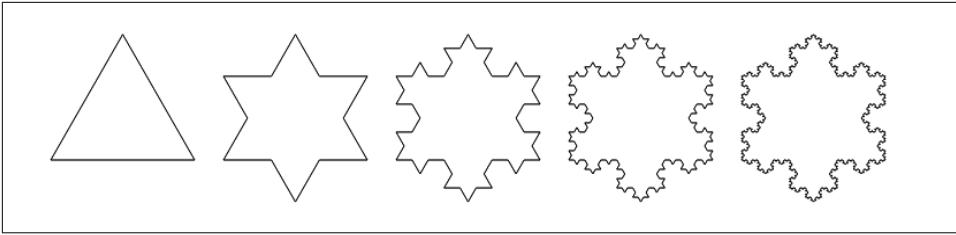
Figure 15-12. Koch snowflakes
