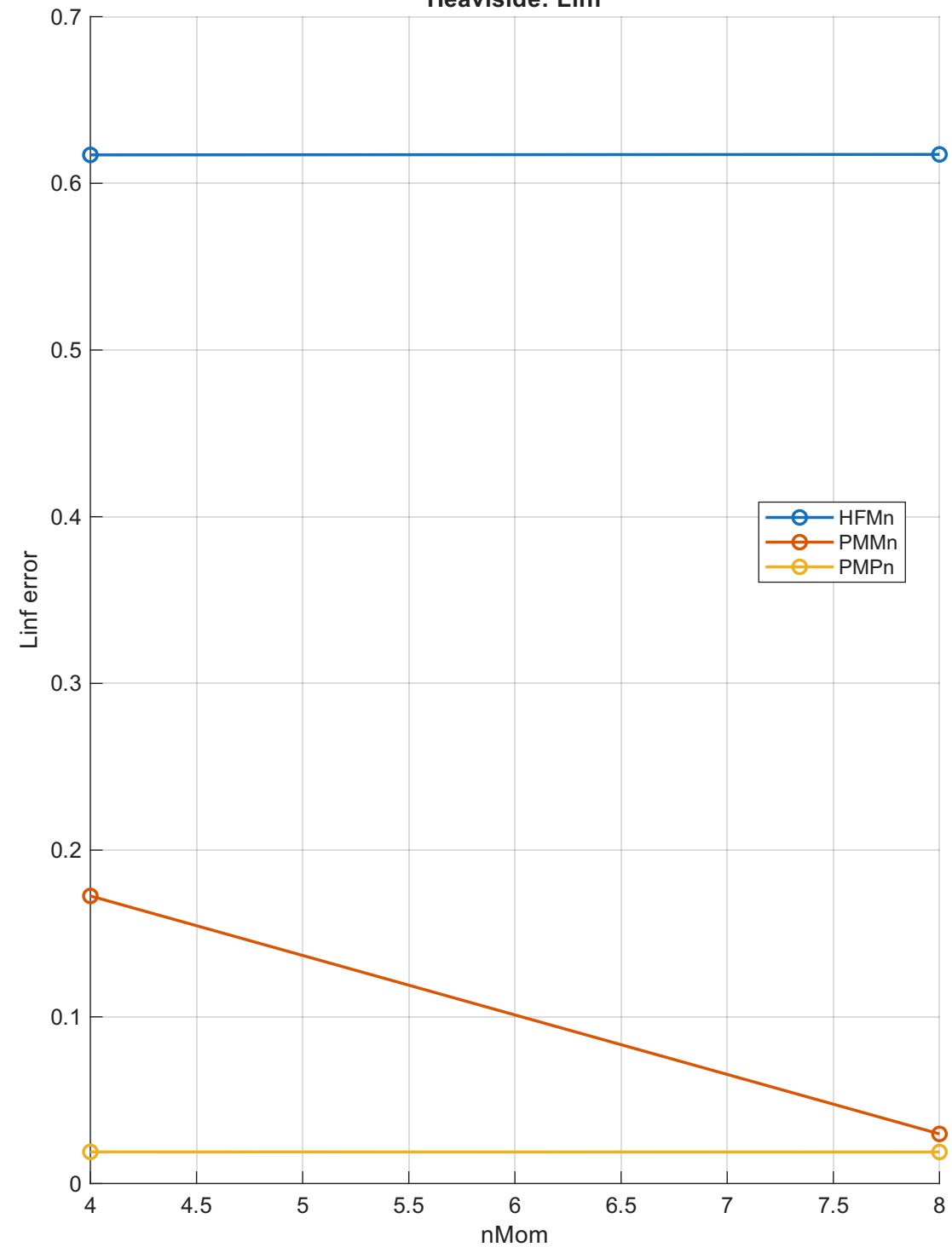
Heaviside: Linf
