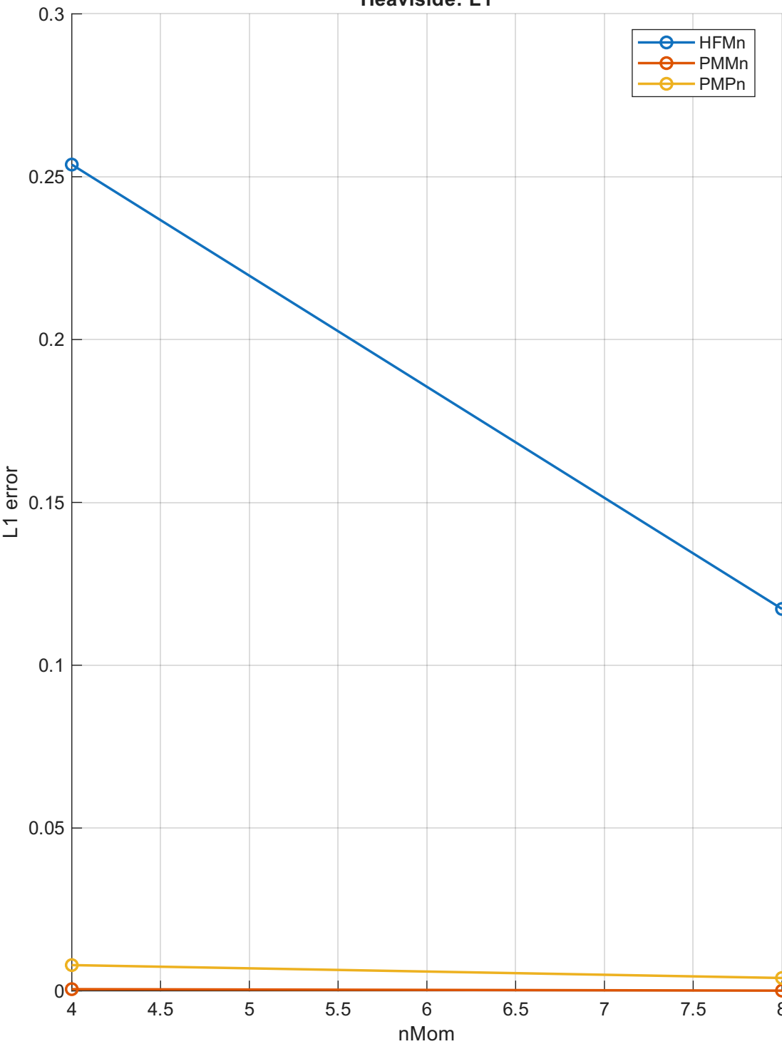
Heaviside: L1
