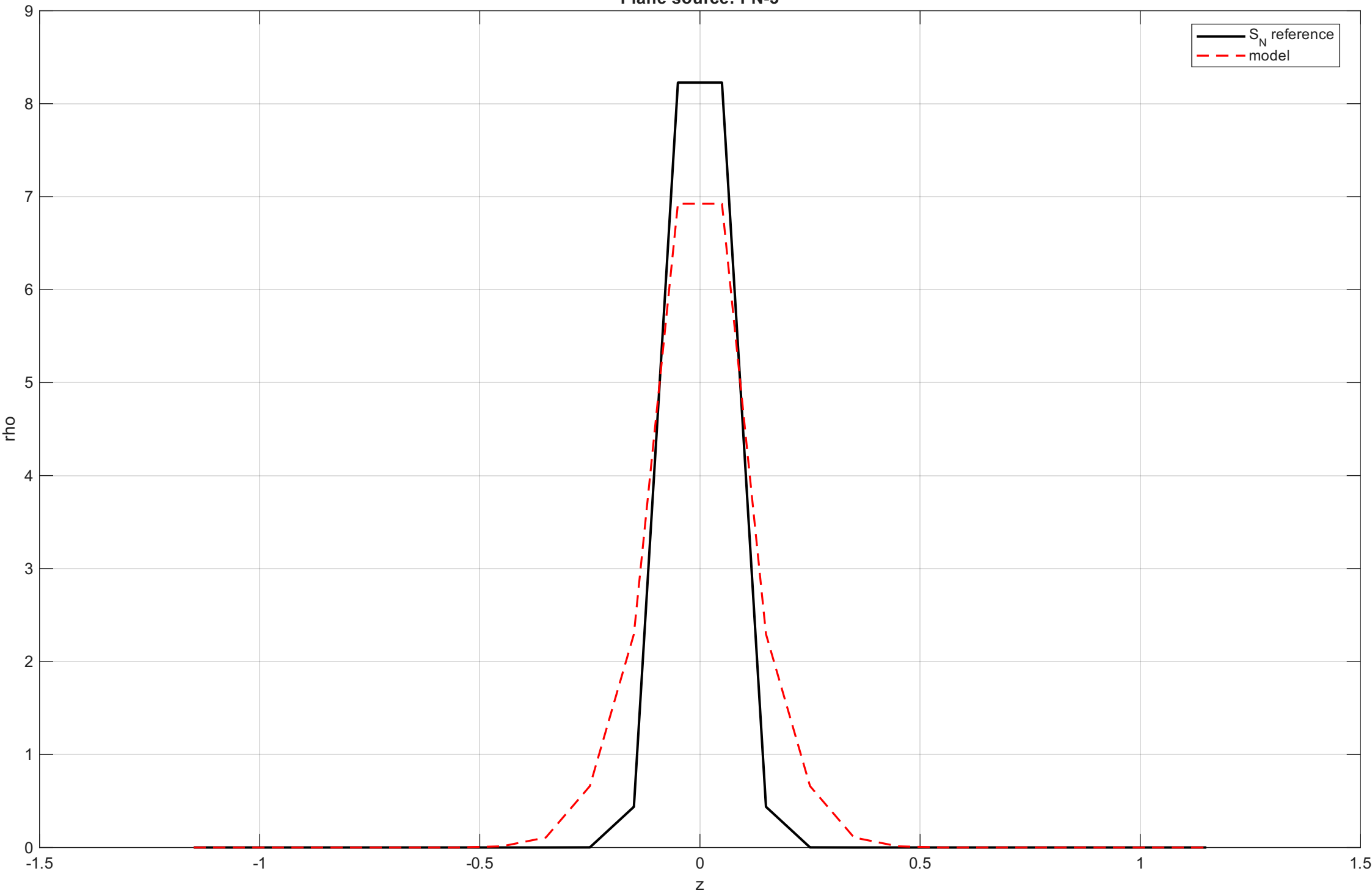
Plane source: PN-3
