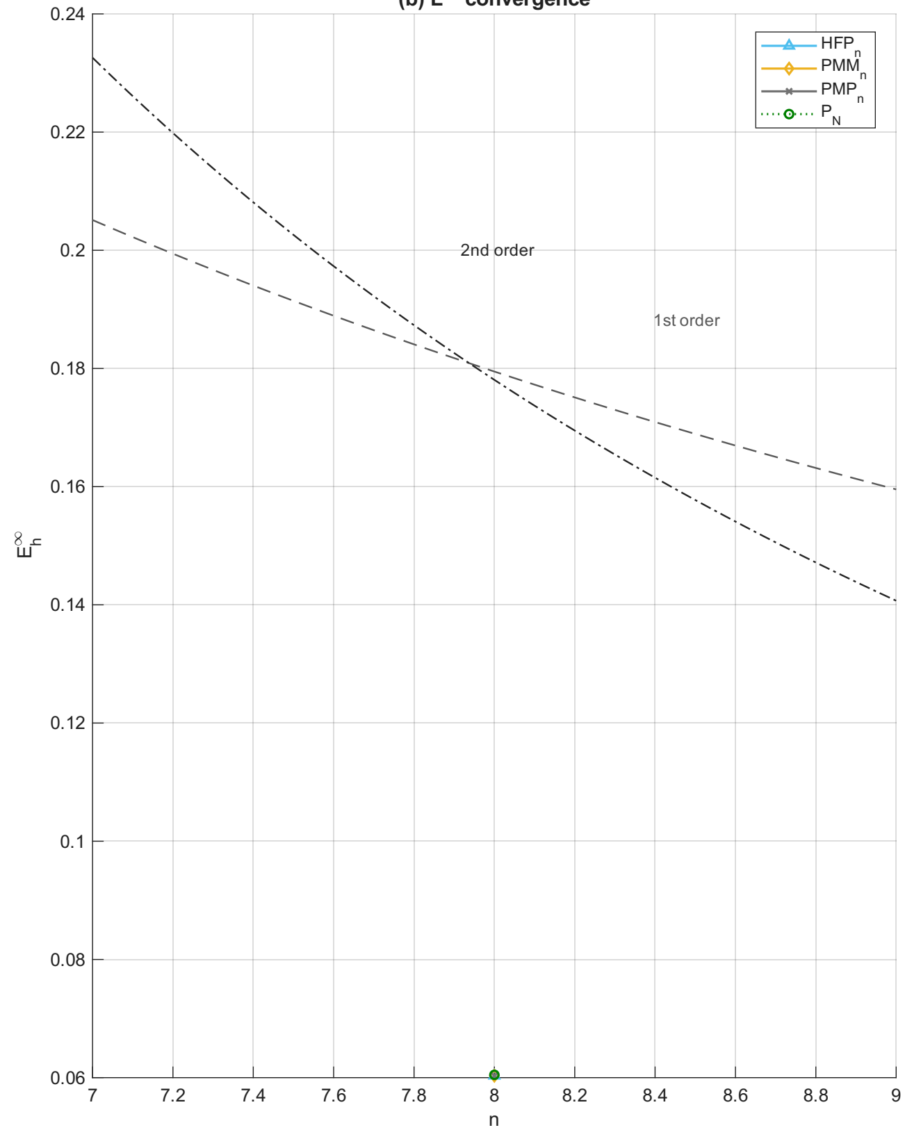
(b) L^\infty convergence
