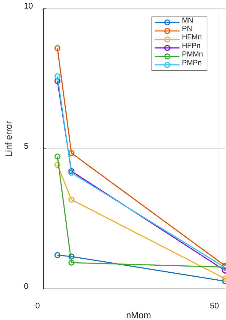
Plane source Linf error
