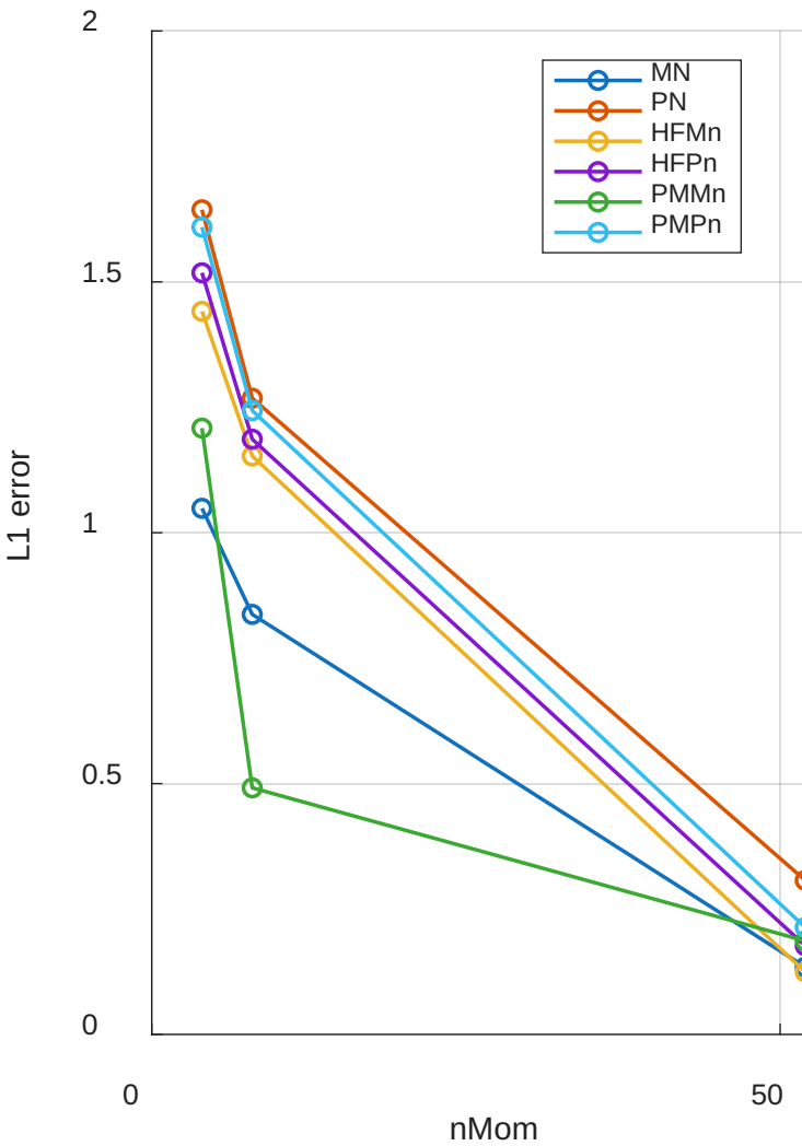
Plane source L1 error
