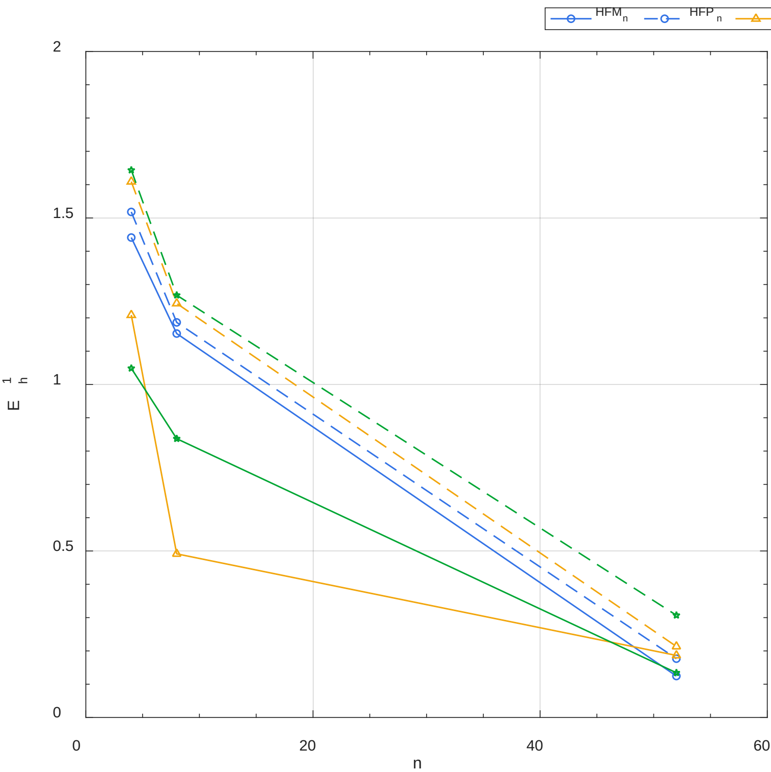
(a) \ell^1 convergence
