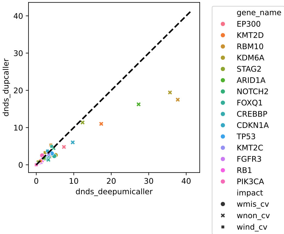
dNdScv dN/dS comparison between DeepUMICaller and DupCaller
