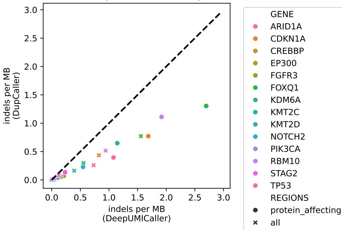
indels mutation density comparison between deepUMIcaller and DupCaller
