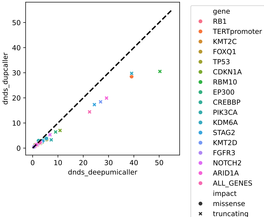
Omega globalloc dN/dS comparison between DeepUMICaller and DupCaller
