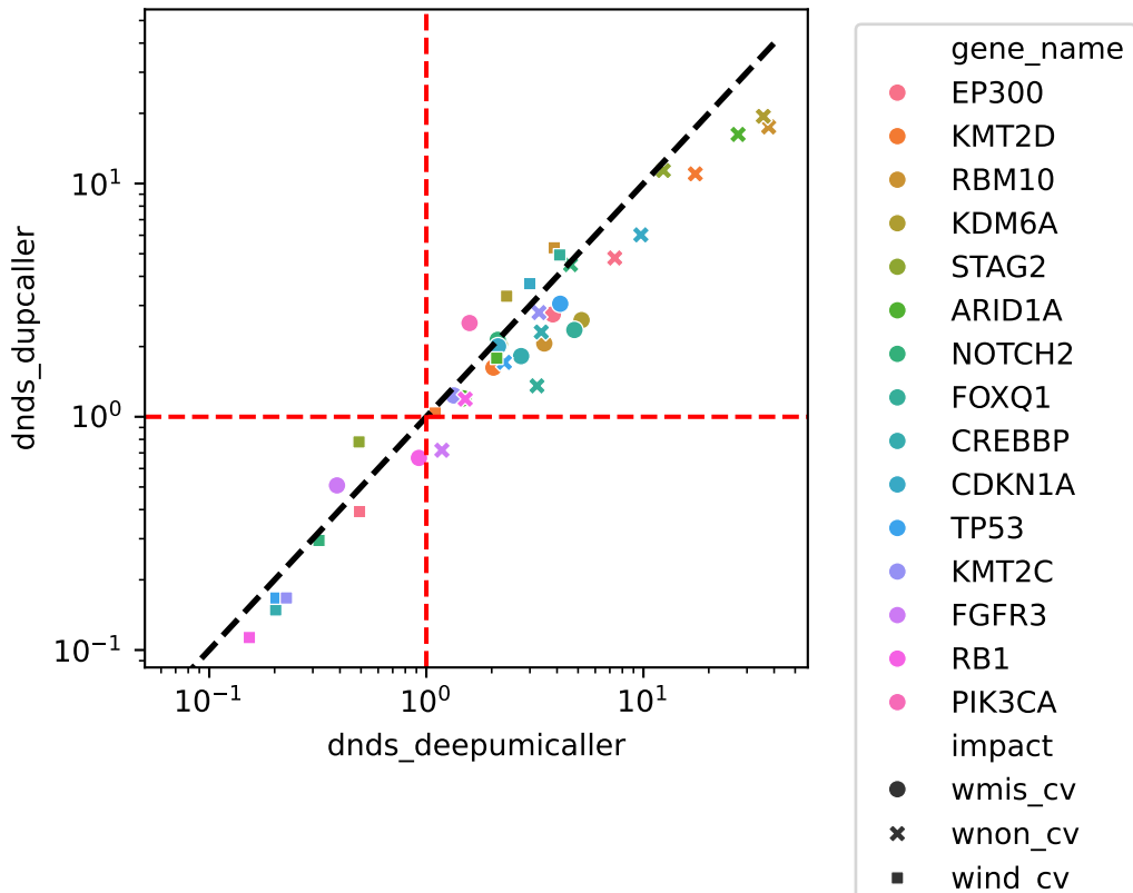
dNdScv dN/dS comparison between DeepUMICaller and DupCaller
