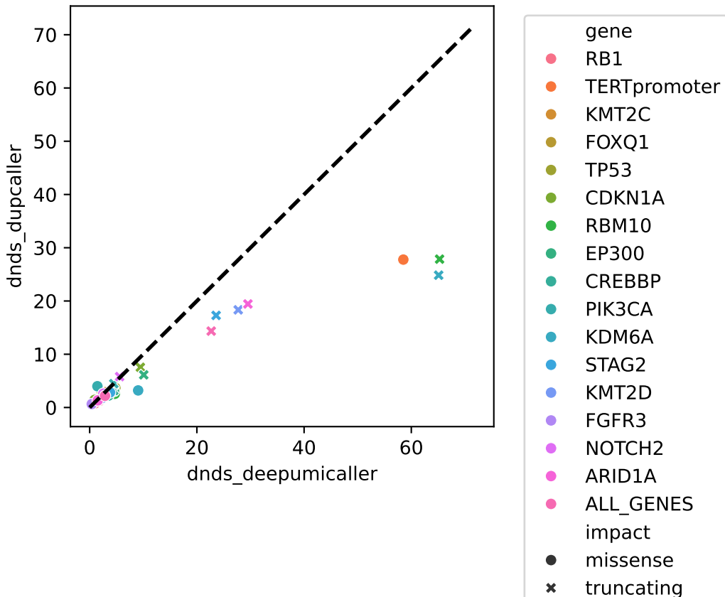
Omega dN/dS comparison between DeepUMICaller and DupCaller
