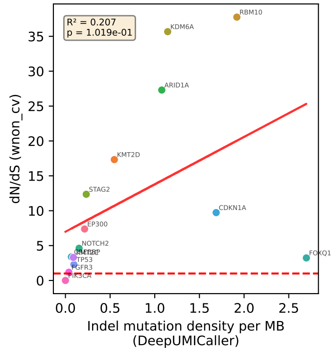
Indel mutation density vs dN/dS
