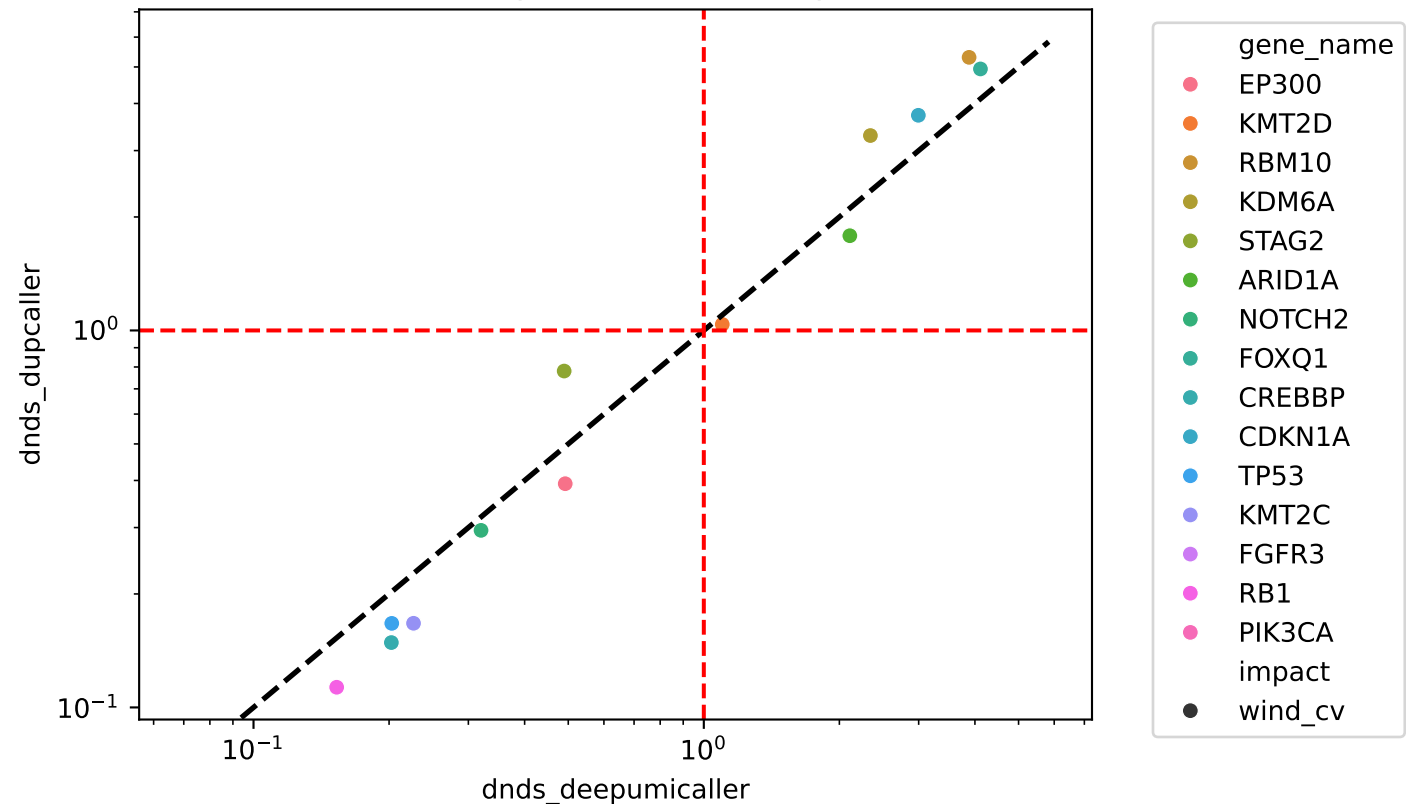
dNdScv indel dN/dS comparison between DeepUMICaller and DupCaller
