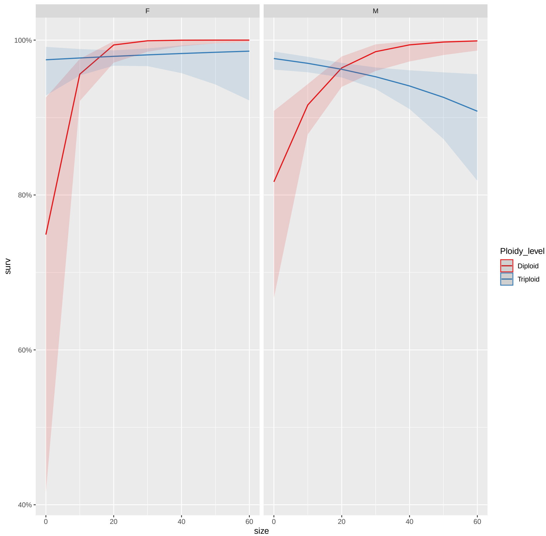
Predicted probabilities of surv
