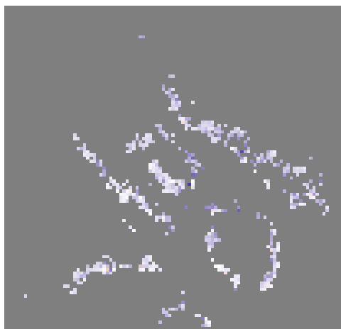
basal_area_density_final
