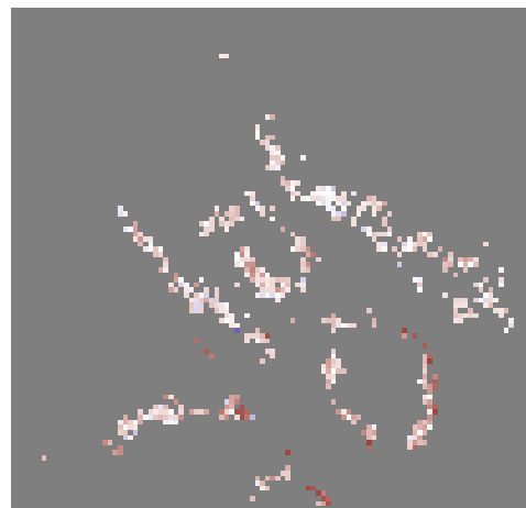
n_S _final
