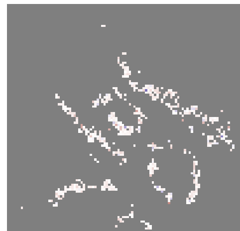
longevity_90_final
