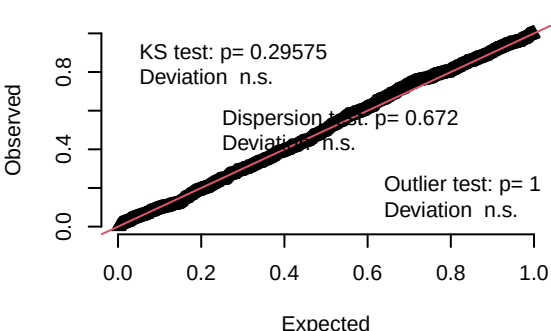
(E) n_R/n_S
