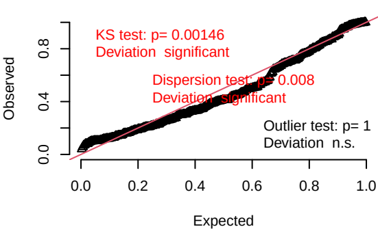
(G) n_S
