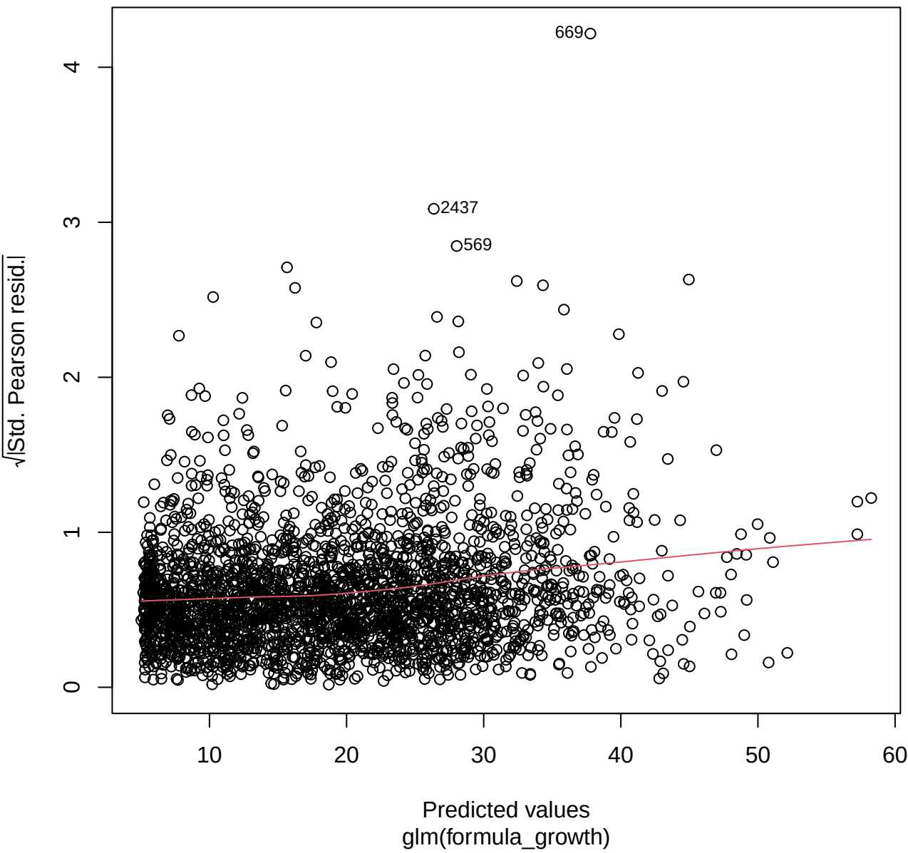
Scale-Location
