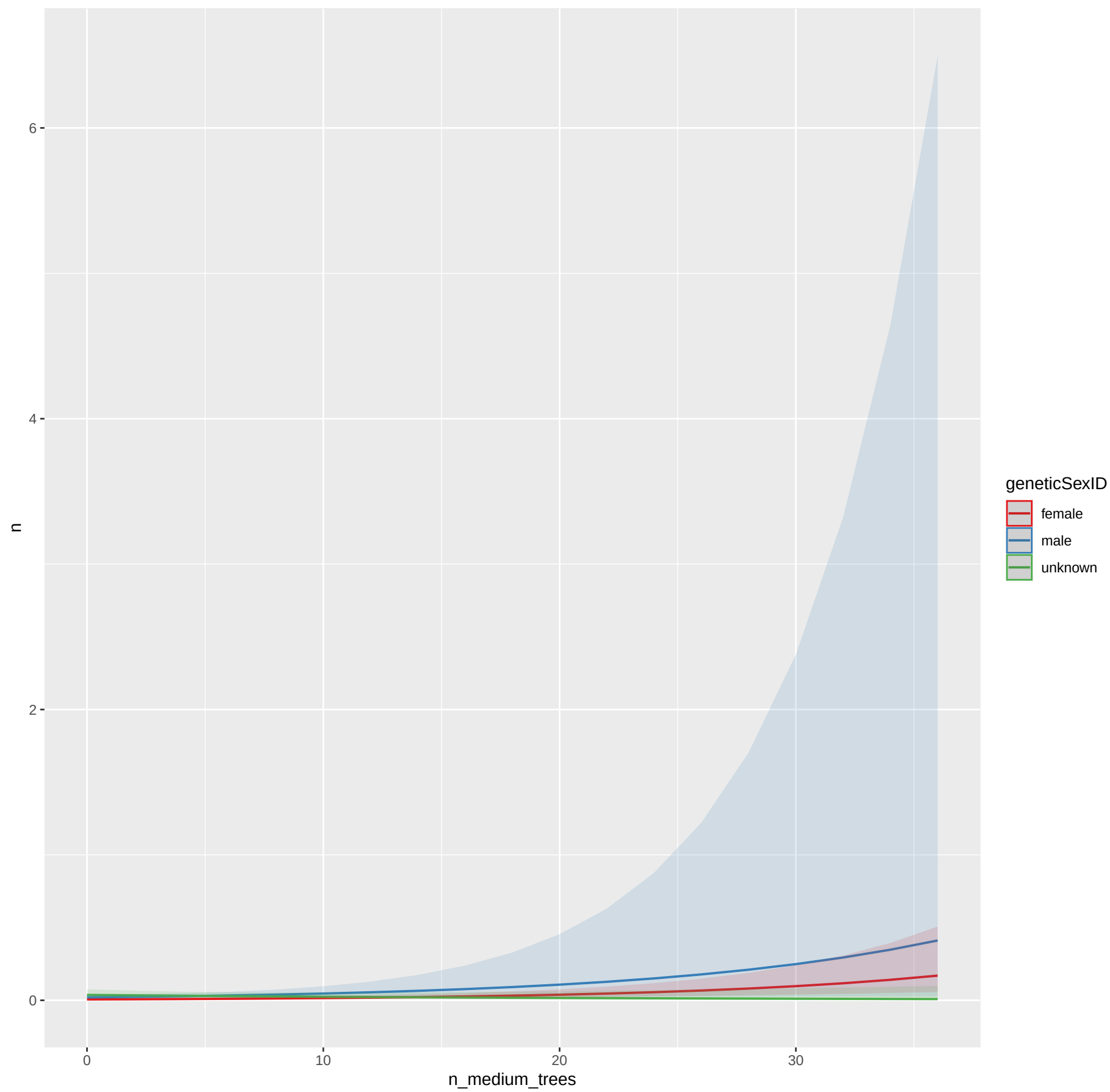
Predicted counts of n
