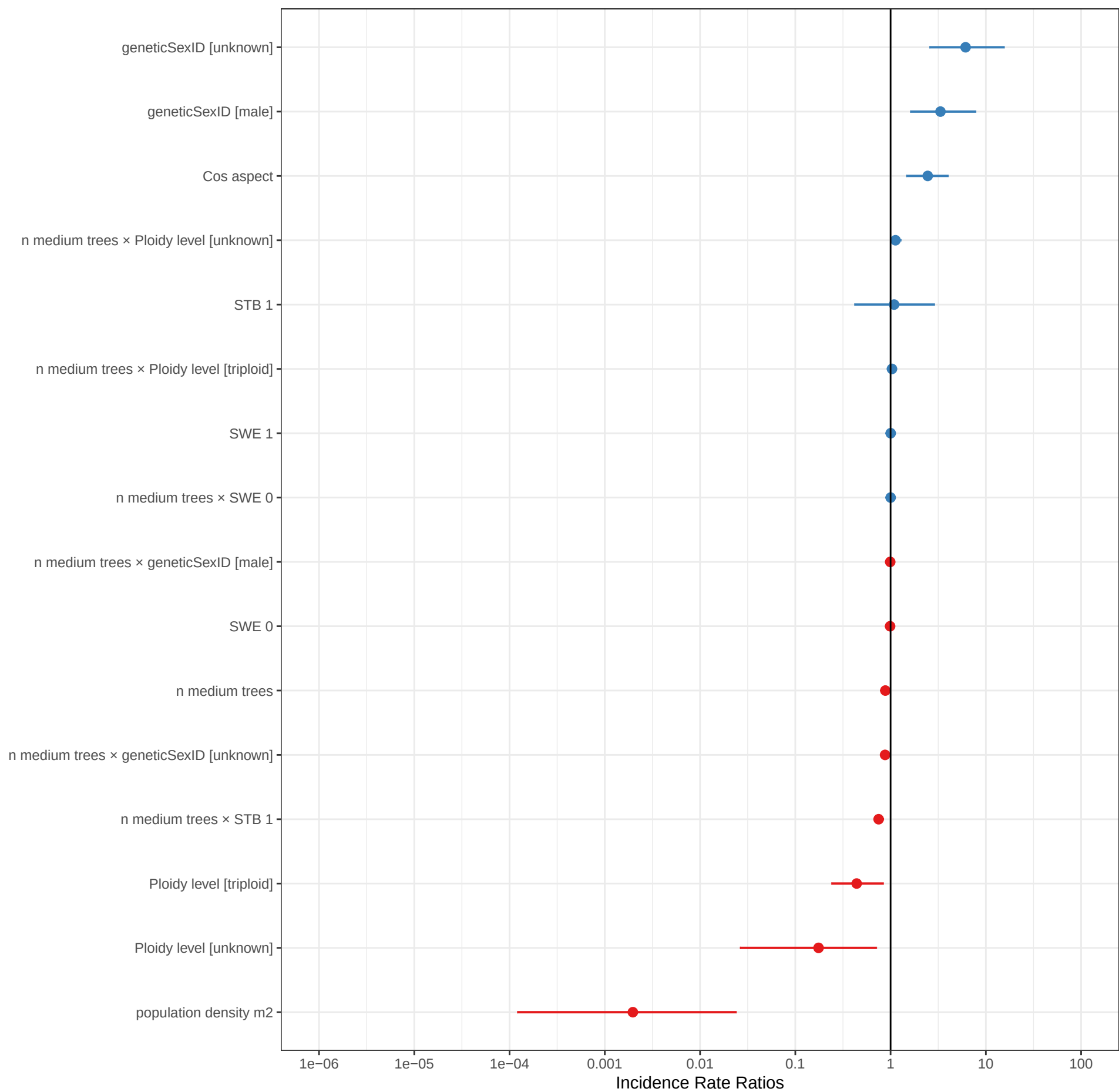
recruit count, standardized effect
