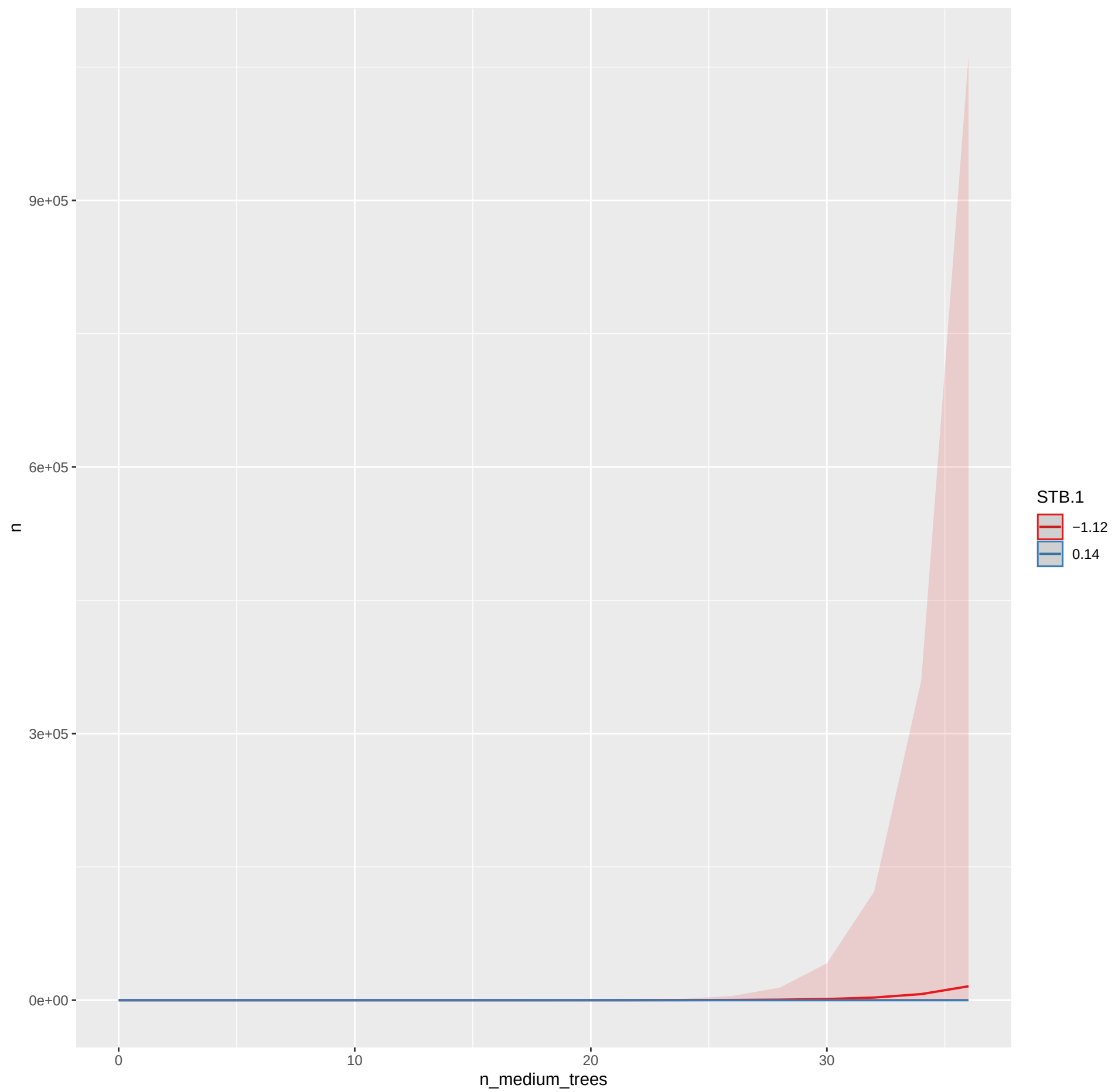
Predicted counts of n
