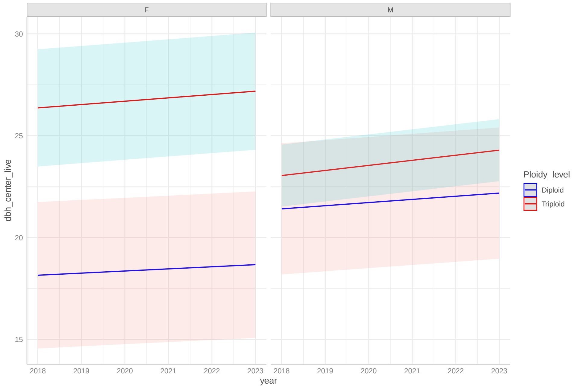
Predicted values of dbh_center_live
