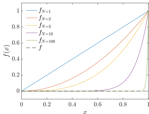
Figure 3.1: Convergence of f_N(x) = x^N .
