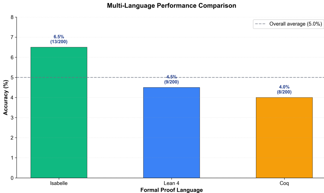
Figure 2: WayneIA Performance Across Formal Languages. Isabelle (6.5%) outperforms Lean 4 (4.5%) and Coq (4.0%), contrary to the Lean-centric focus in current research.
