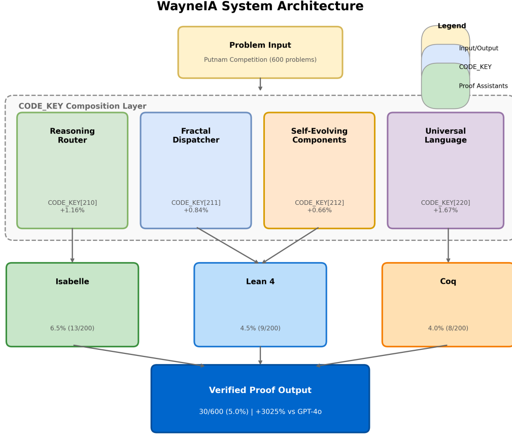
Figure 1: WayneIA System Architecture with CODE_KEY[220] Universal Language Transformer. The multi-level design includes: Input Layer (mathematical statement intake), Reasoning Router (task complexity analysis), Universal Language Transformer (multi-language encoding), Agent Swarm (7 production agents, 147KB total), and Output Layer (verified formal proofs).
