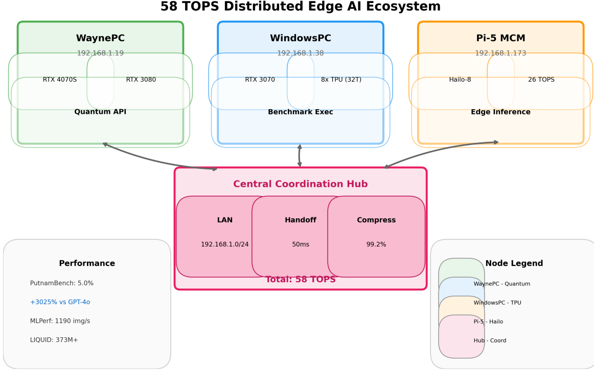
Figure 2: 84 TOPS Distributed Ecosystem Architecture. Three nodes coordinate via the PPWHH protocol: WaynePC (Quantum API, dual GPU), WindowsPC (32 TOPS via 8x Coral TPU), and Pi-5 MCM (26 TOPS Hailo-8 edge inference). Context compression achieves 99.2% efficiency with <50ms hot-handoff latency.
