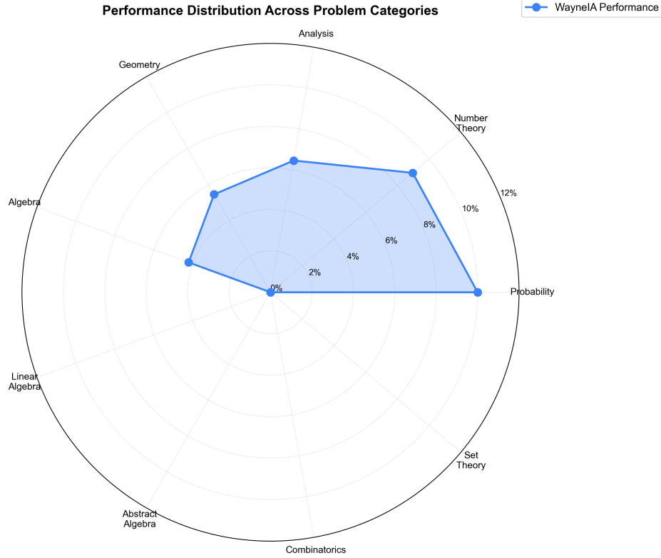
Figure 3: Performance Distribution Across Problem Categories. Peak accuracy in Probability (10.0%) and Number Theory (8.96%), with zero performance in Linear/Abstract Algebra, Combinatorics, and Set Theory indicating areas for improvement.
