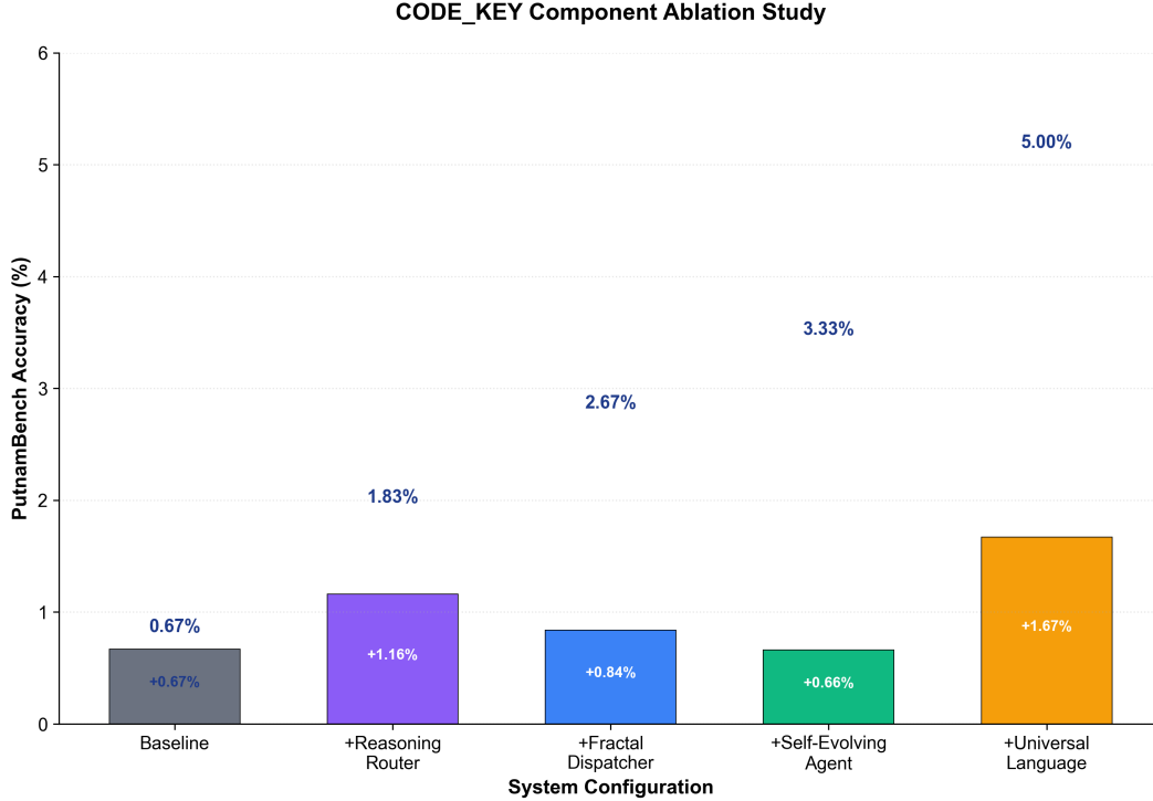
Figure 6: Incremental Contribution of CODE_KEY Components. The Universal Language Transformer provides the largest single improvement (+1.67%), followed by the Reasoning Router (+1.16%), Fractal Dispatcher (+0.84%), and Self-Evolving Agent (+0.66%).
