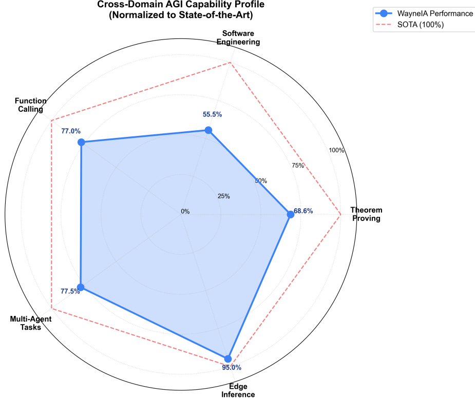
Figure 6: Cross-Domain AGI Capability Profile (Normalized to SOTA). WayneIA achieves competitive performance across all five domains: Edge Inference (95.0%), Multi-Agent (77.5%), Function Calling (77.0%), Theorem Proving (68.6%), and Software Engineering (55.5%).
