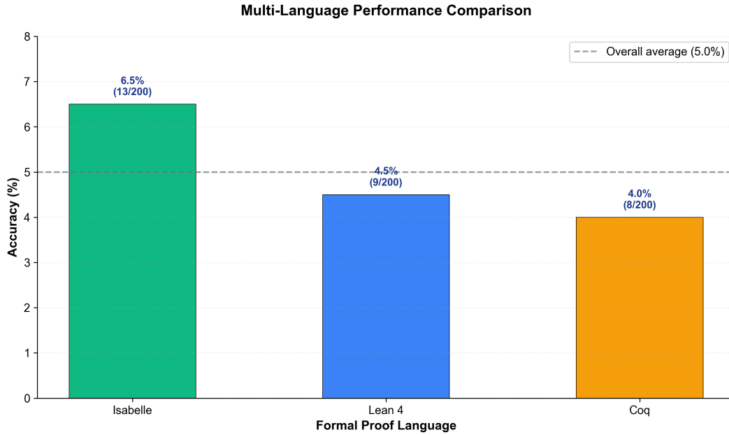
Figure 3: WayneIA Performance Across Formal Languages. Isabelle (6.5%) outperforms Lean 4 (4.5%) and Coq (4.0%), contrary to the Lean-centric focus in current research.
