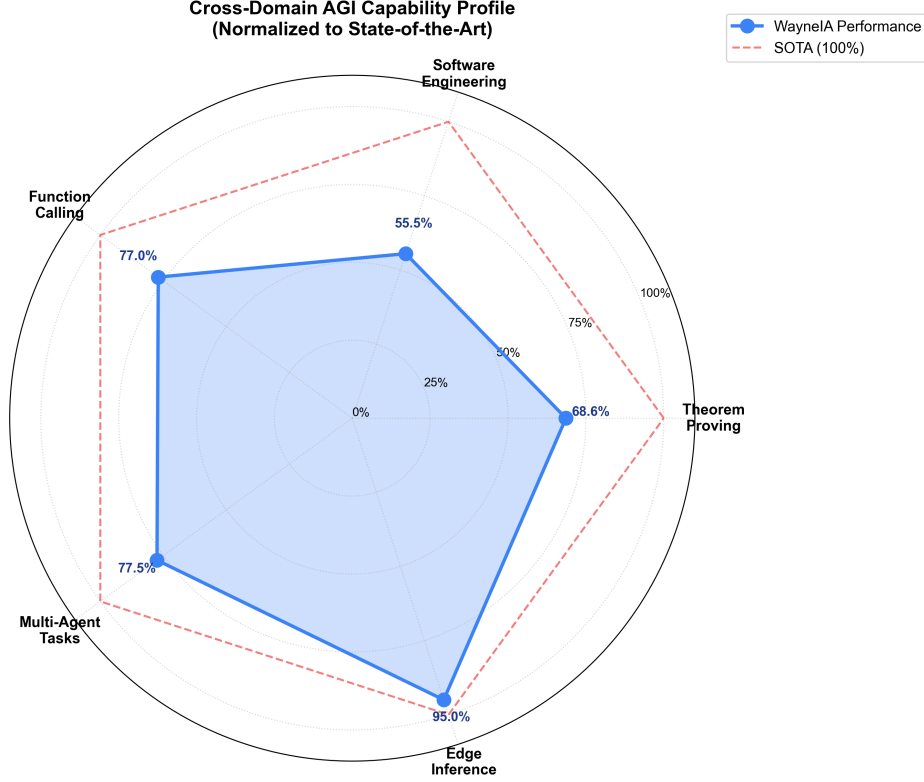
Figure 7: Cross-Domain AGI Capability Profile (Normalized to SOTA). WayneIA achieves competitive performance across all five domains: Edge Inference (95.0%), Multi-Agent (77.5%), Function Calling (77.0%), Theorem Proving (68.6%), and Software Engineering (55.5%).
