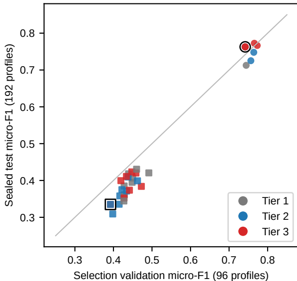
Selected prompts
