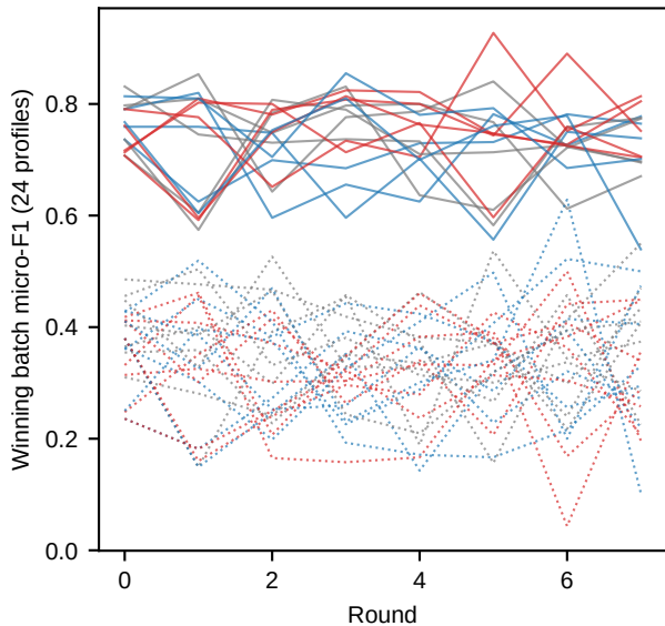
Search dynamics
