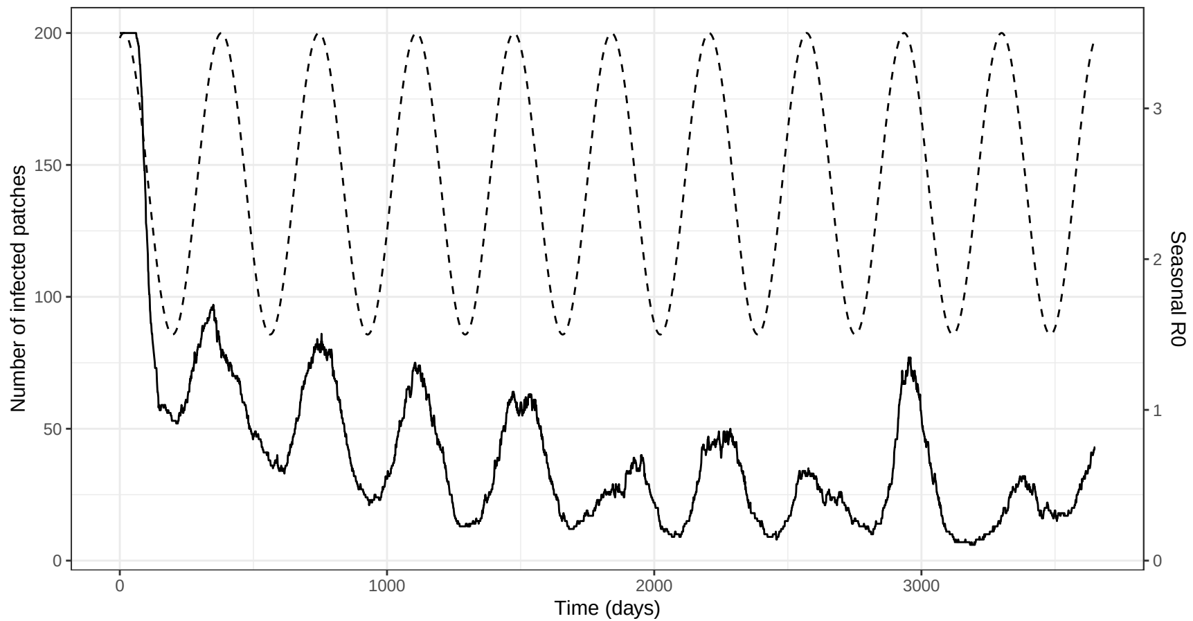
Patch occupancy and seasonal transmission
