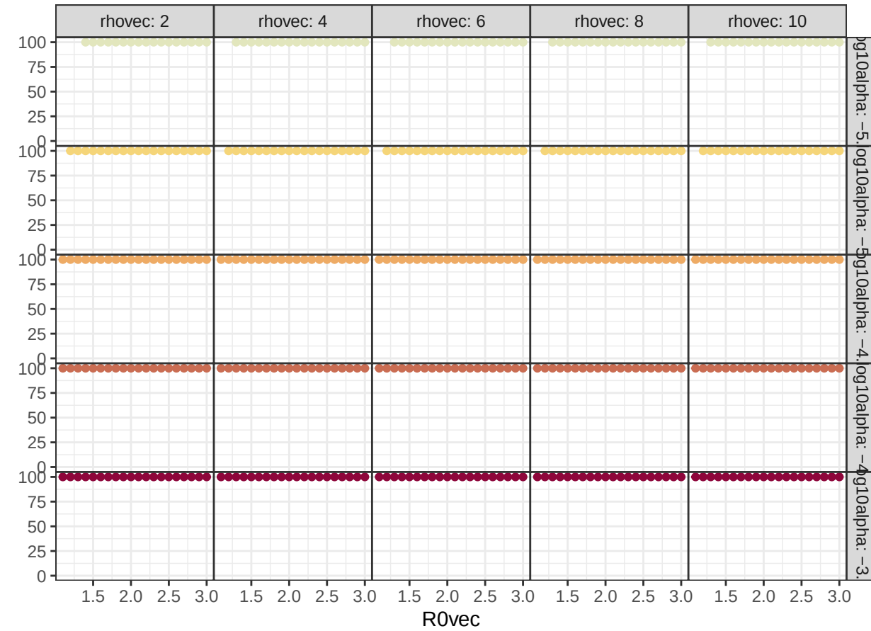
Total host population (x 1e6; quasi-eq)
