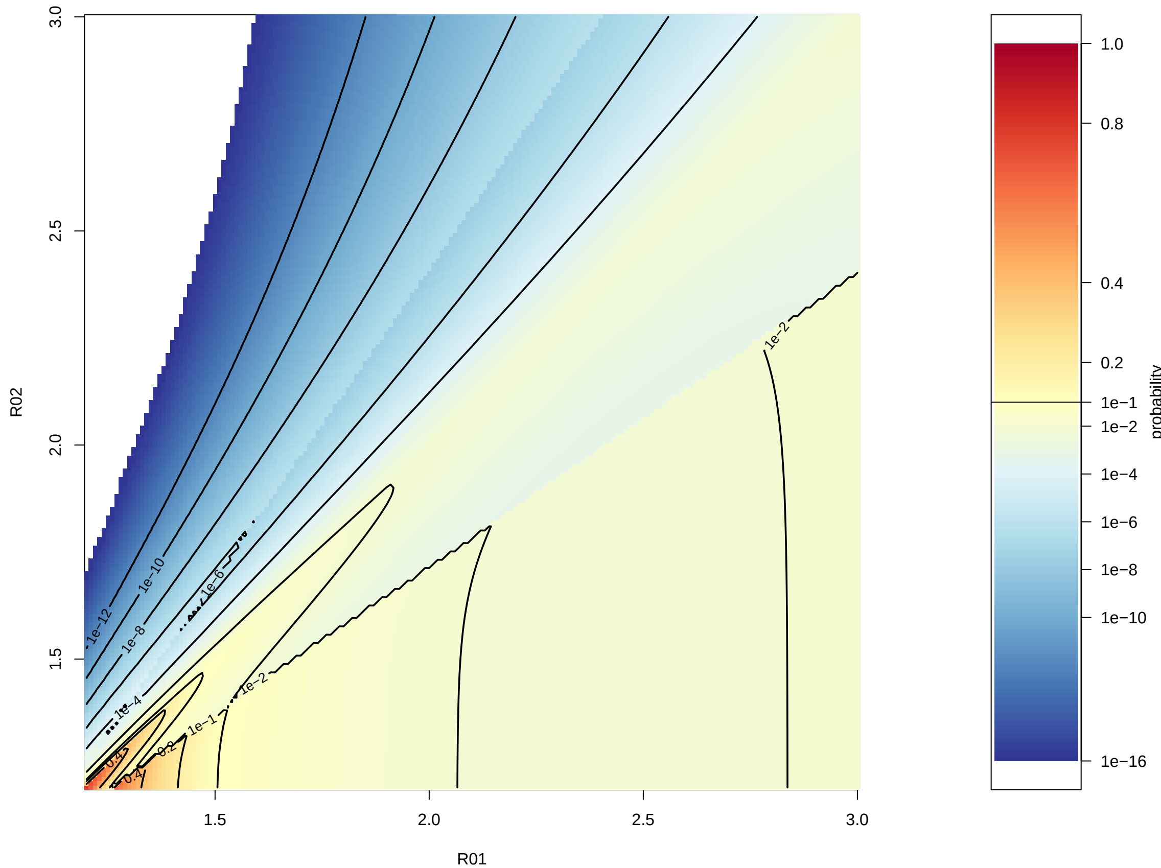
Strain 1 persistence probability: 1 - Q_1
