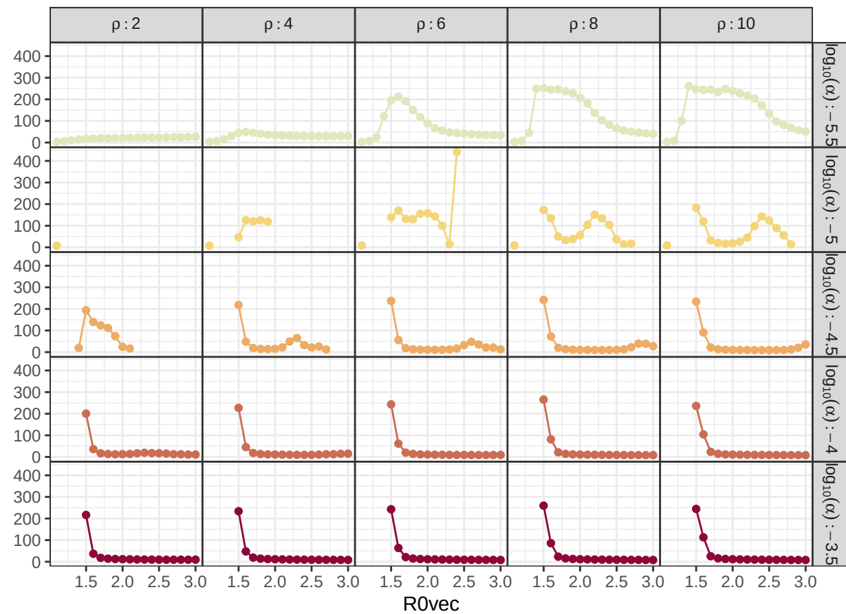
Infected patches (quasi-eq)
