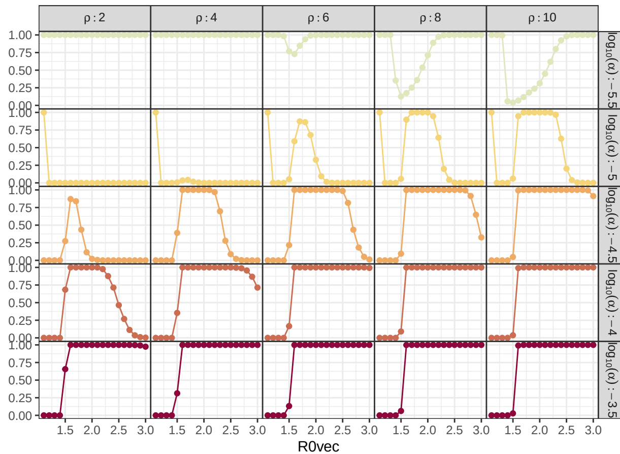
Total Infections (x 1e6; quasi-eq)
