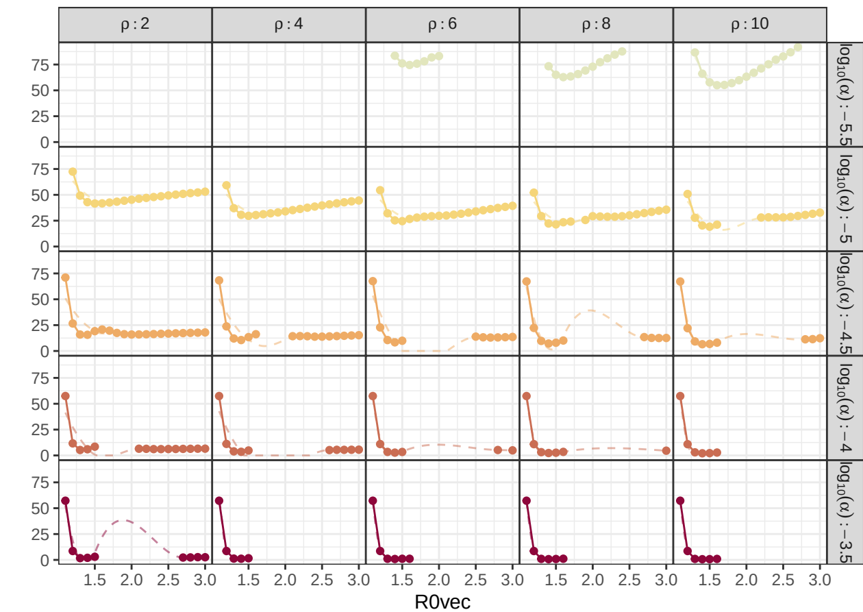
Total host population (x 1e6; quasi-eq)
