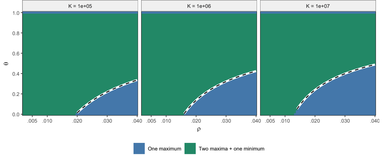
Figure 6: Unconditional-persistence shape maps for K = 10^5, 10^6, 10^7 , classified as in ???. The dashed line in each panel is the genuine G = G_{\mathcal{R}_0} = 0 pair-creation locus. Higher K moves this boundary toward larger \theta ; the endpoint \theta = 1 remains a one-maximum curve over the displayed \rho range.
