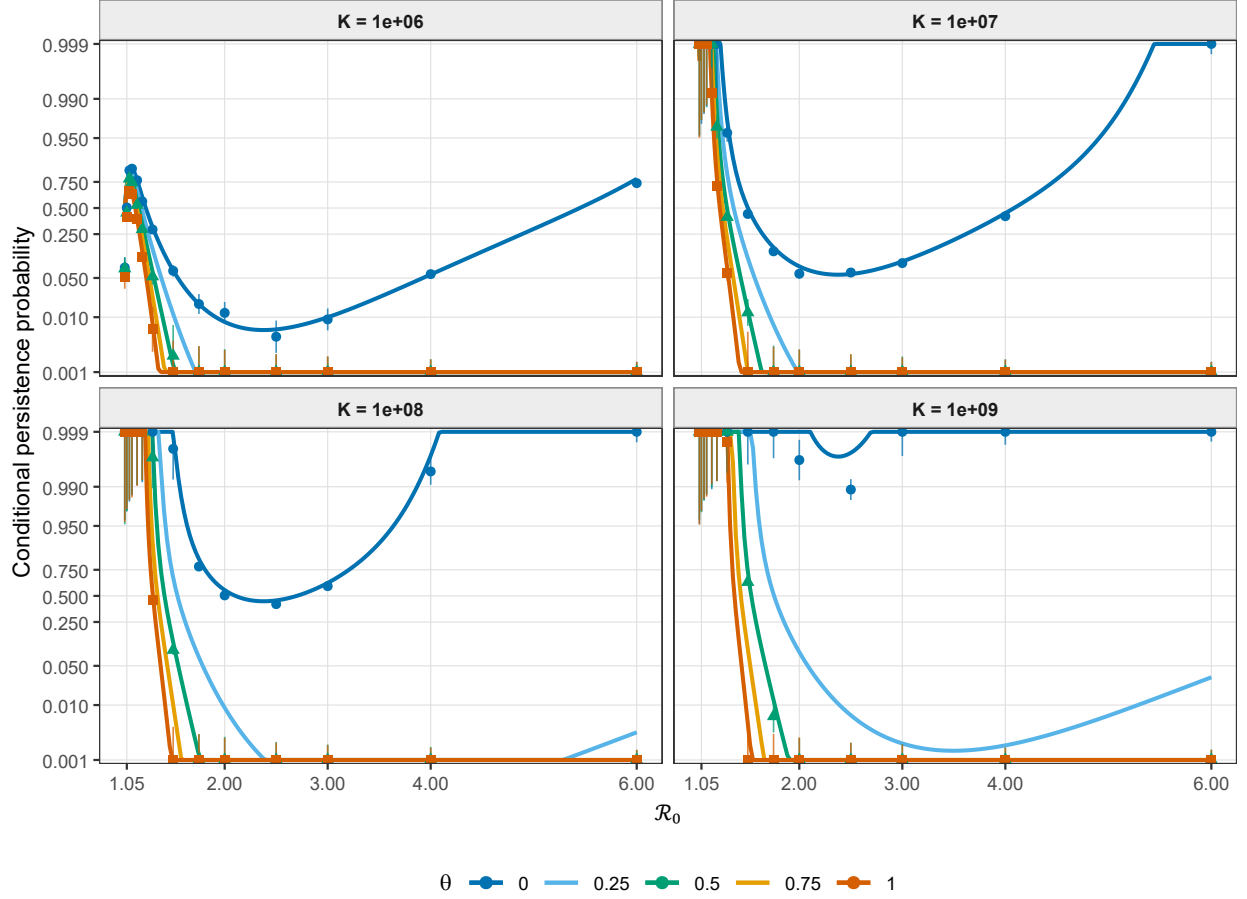
Figure 1: Conditional persistence after epidemic establishment at \rho = 0.01 . Curves are the boundary-layer-independent prediction ?? for \theta = 0, 0.25, 0.5, 0.75, 1 ; symbols are stochastic estimates for \theta = 0, 0.5, 1 , and vertical bars are 95% Wilson intervals. The probability axis is displayed on logit coordinates so that both tails remain visible; values below 0.001 or above 0.999 are shown at those limits. The adaptive tau-leap scan used 3,000–10,000 attempted epidemics at each point. Agreement is close except at the values nearest \mathcal{R}_0 = 1 , most visibly for K = 10^6 .
