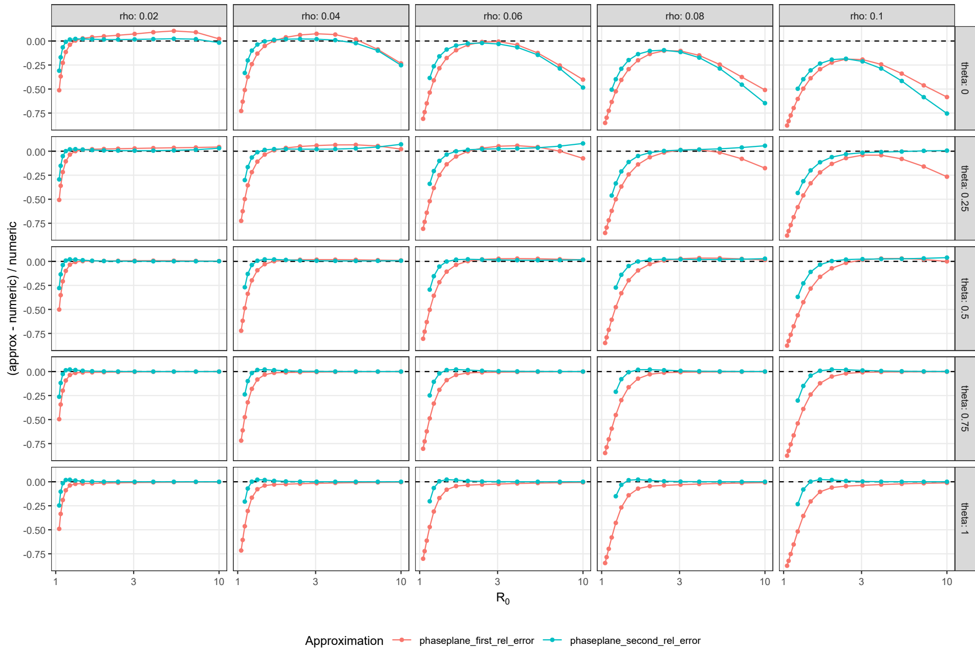
Phase-plane trough approximation error
