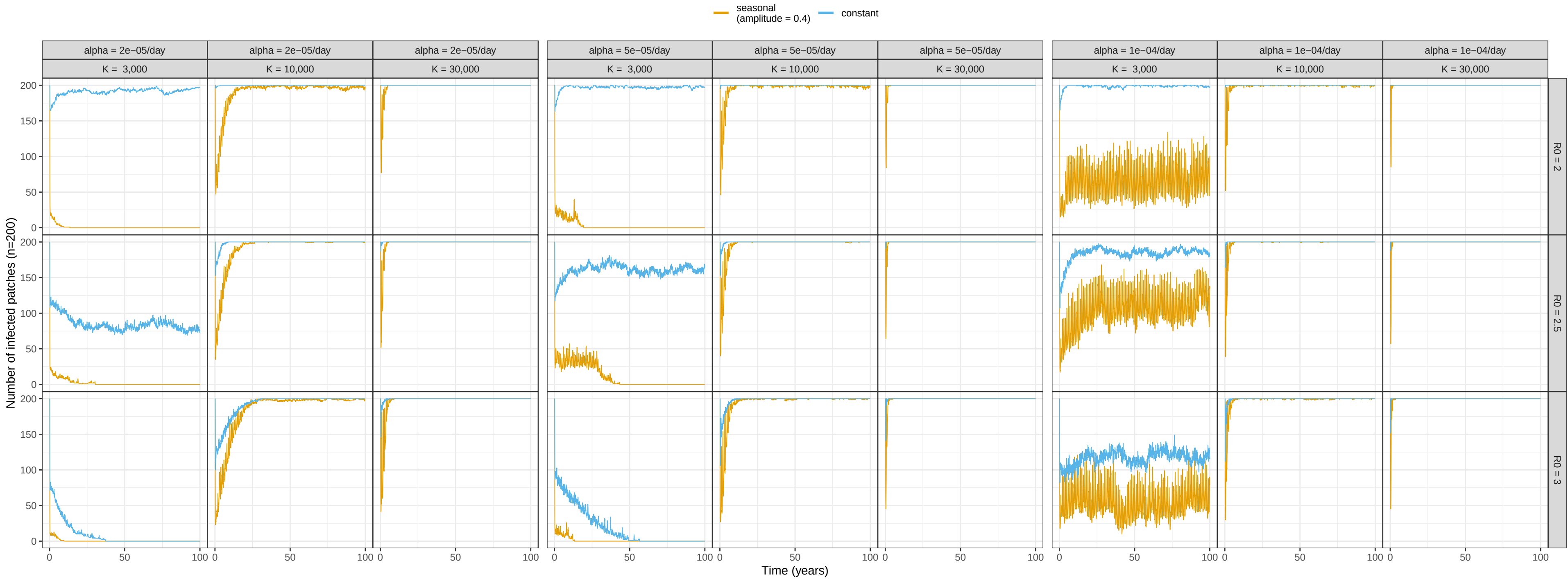
Patch occupancy over 100 years: seasonal vs constant transmission r = 0.025/day, 200 patches, ratchet initial conditions, single realization per panel (seed 101), every 10th day plotted
