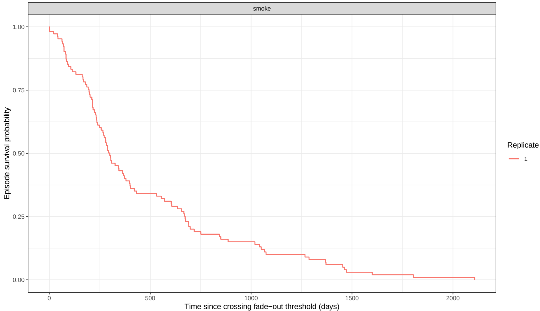
Conditional survival of established infection episodes
