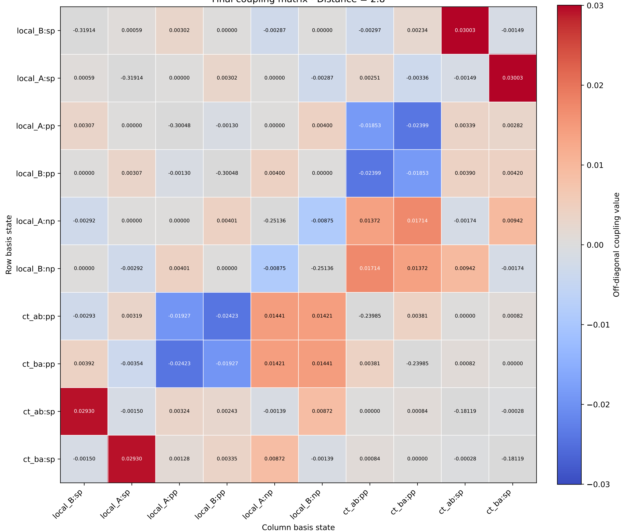
Final coupling matrix - Distance = 2.8
