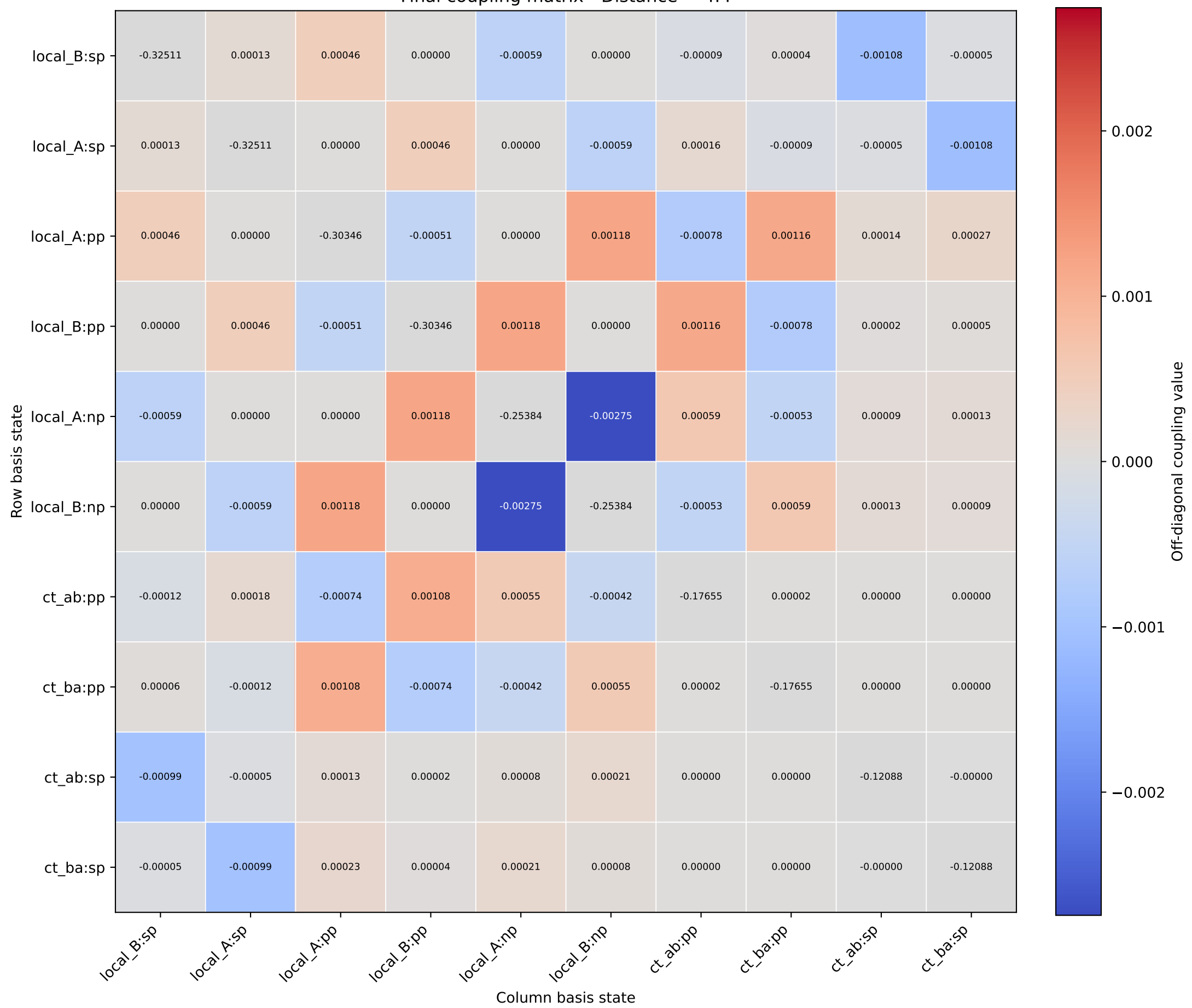
Final coupling matrix - Distance = 4.4
