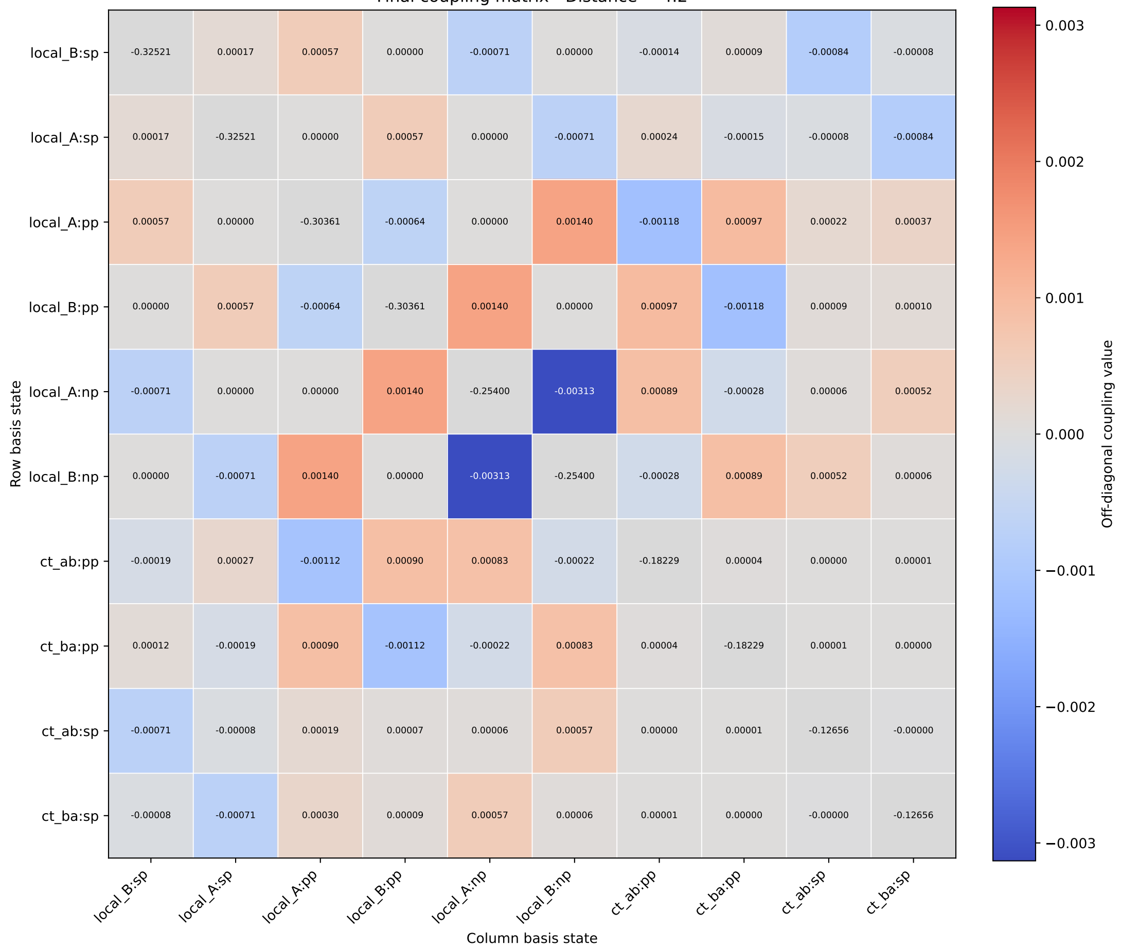
Final coupling matrix - Distance = 4.2
