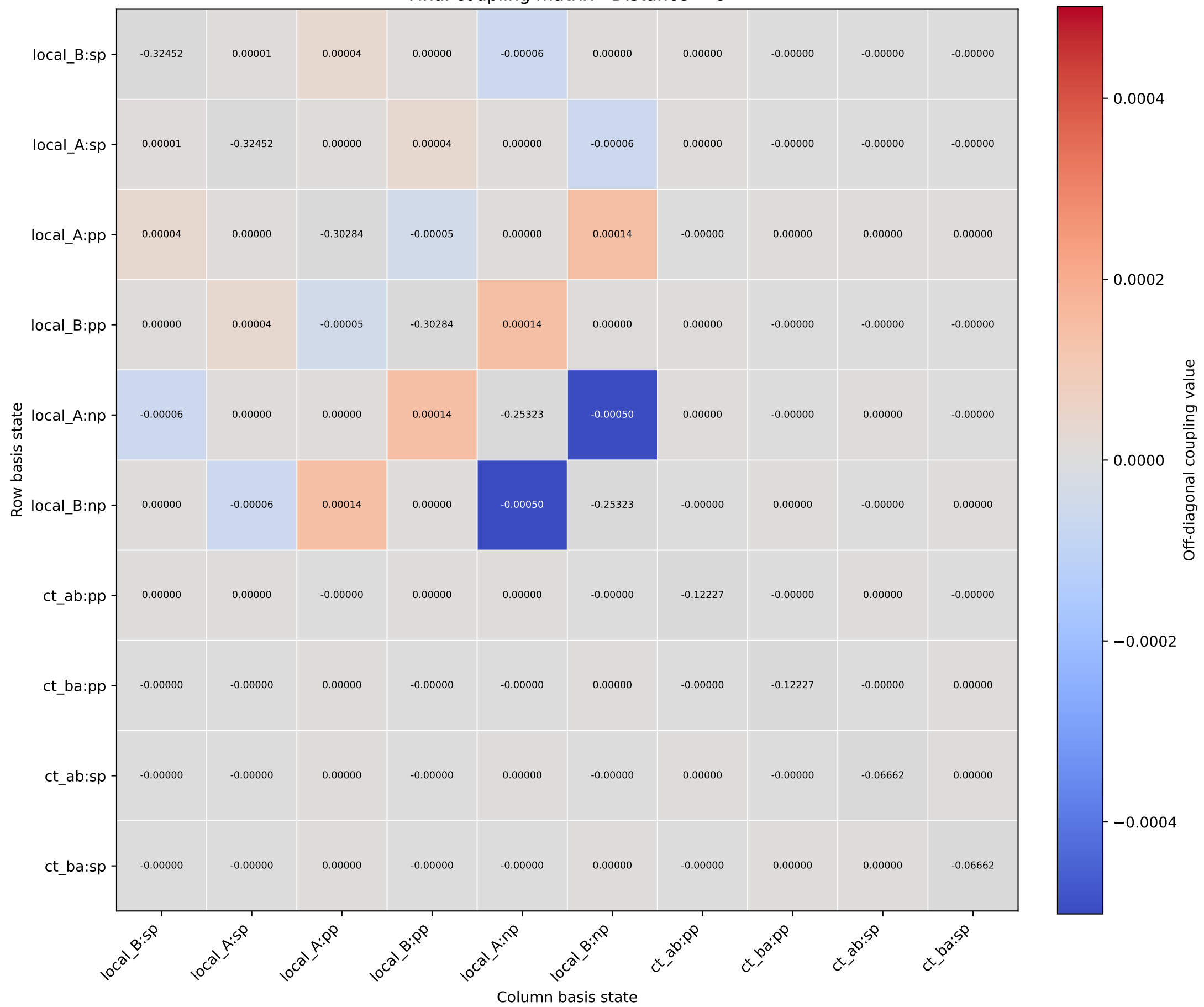
Final coupling matrix - Distance = 8
