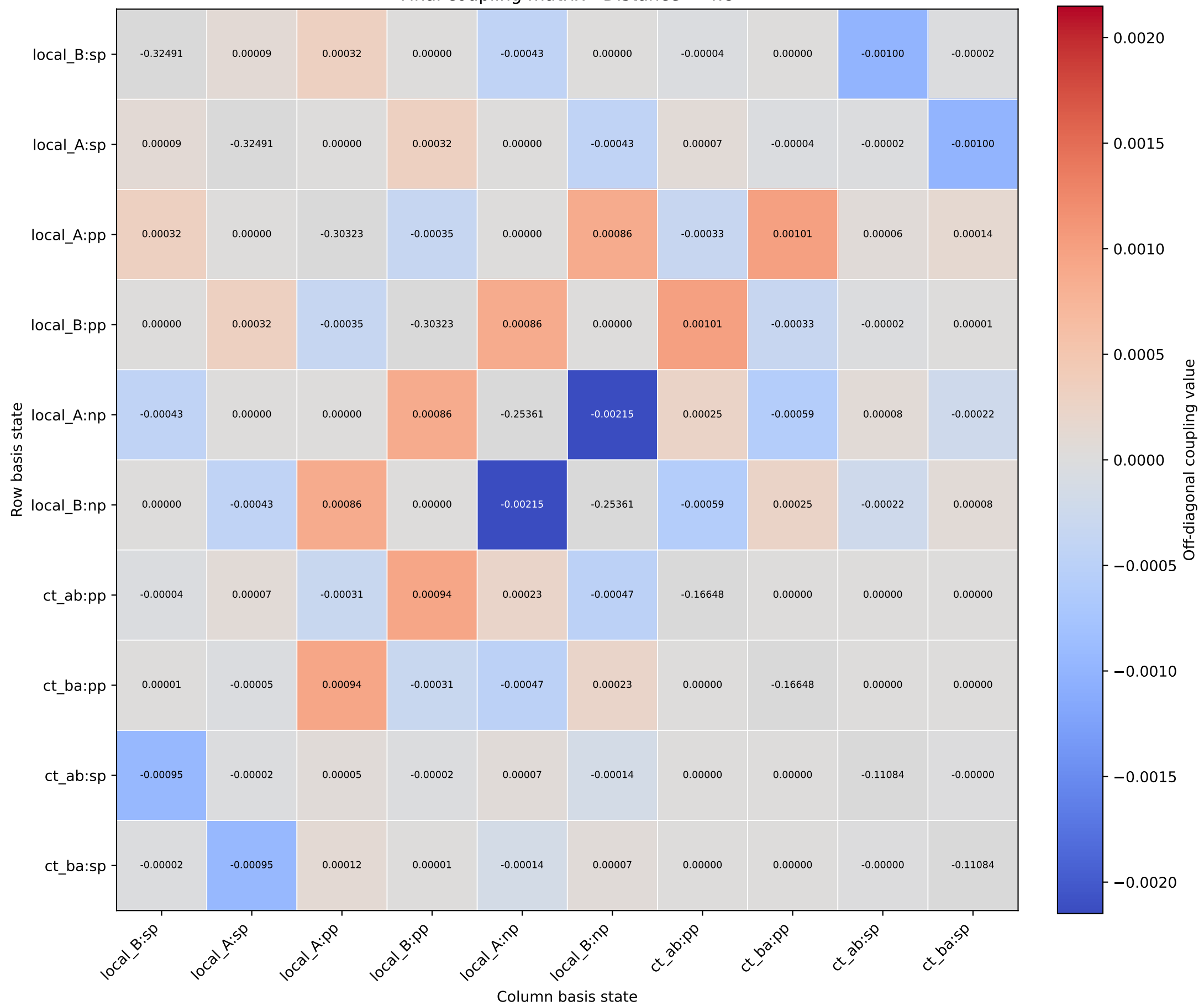
Final coupling matrix - Distance = 4.8
