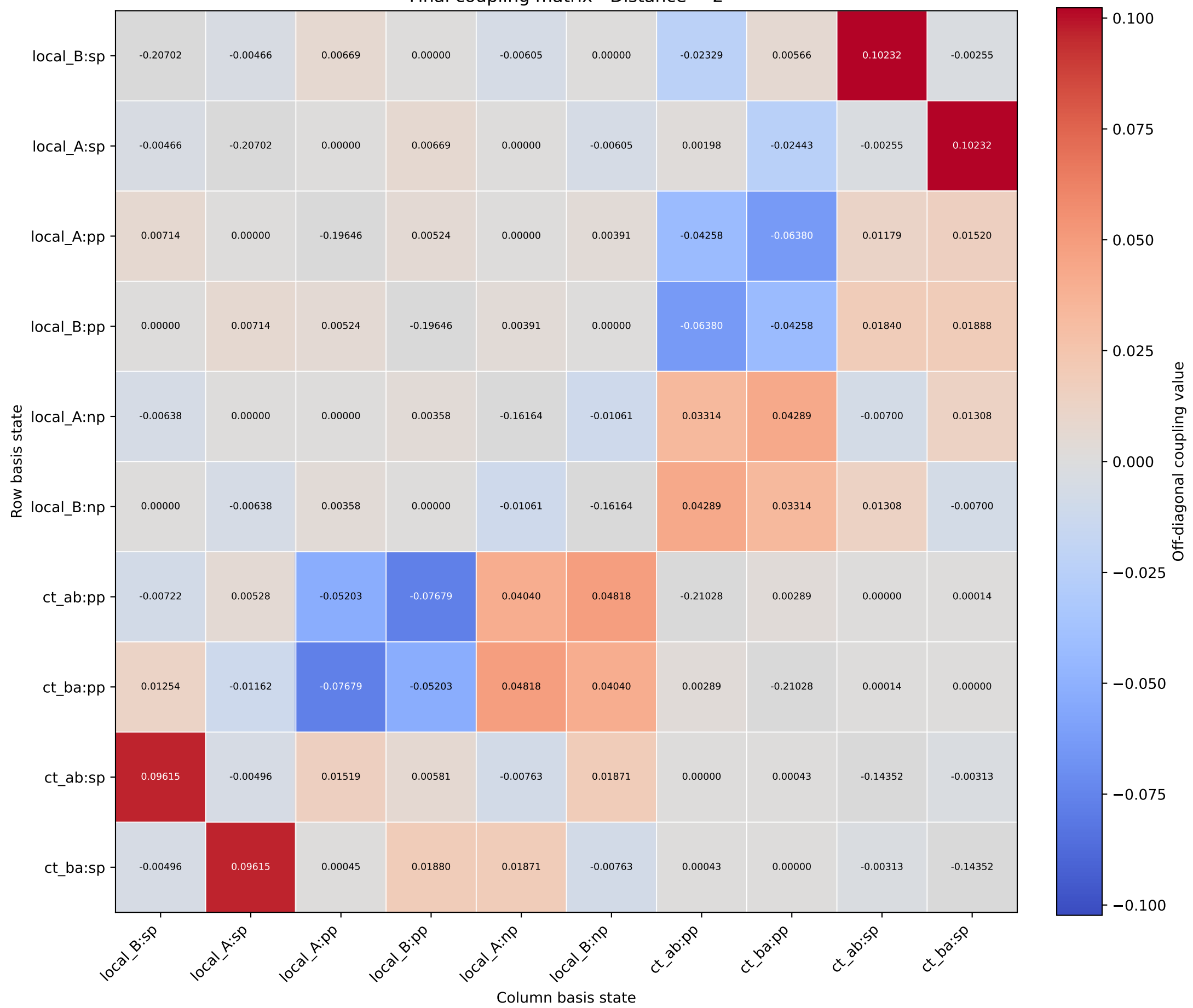
Final coupling matrix - Distance = 2
