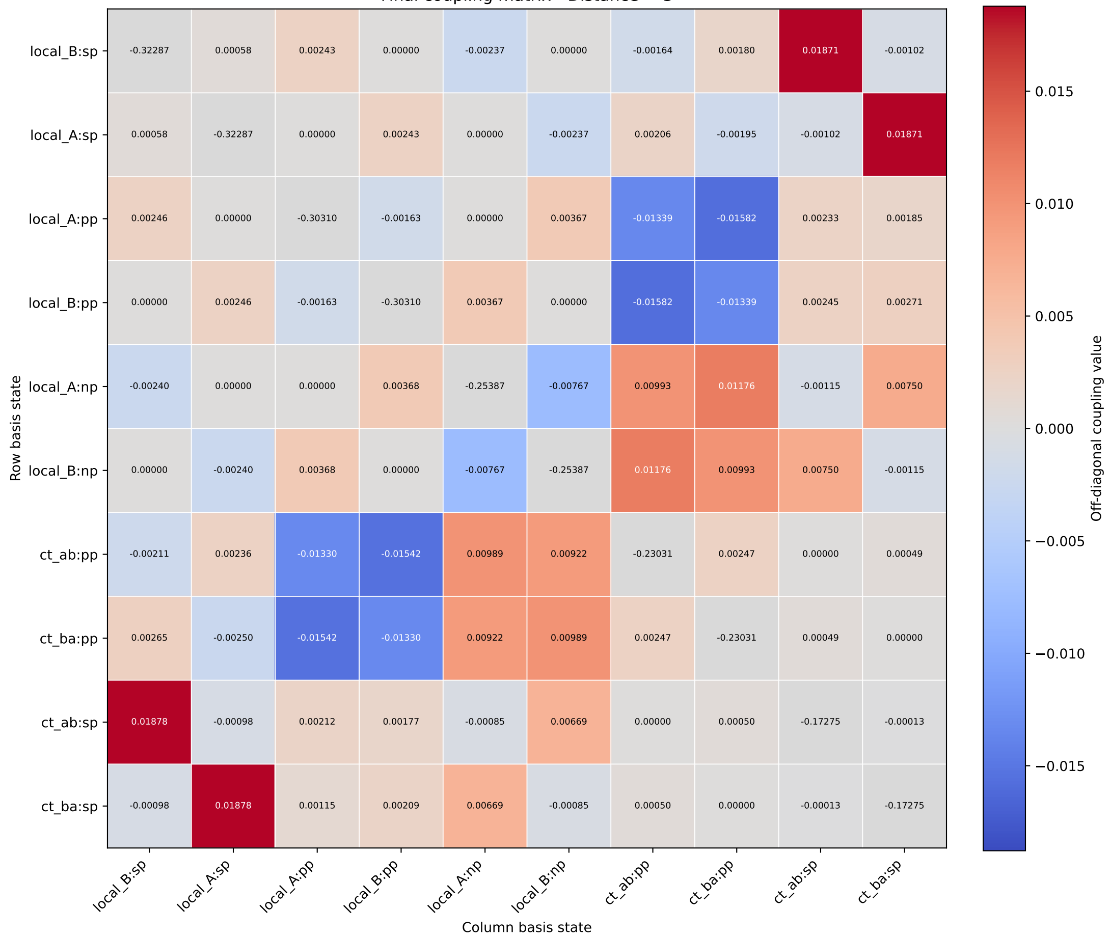
Final coupling matrix - Distance = 3
