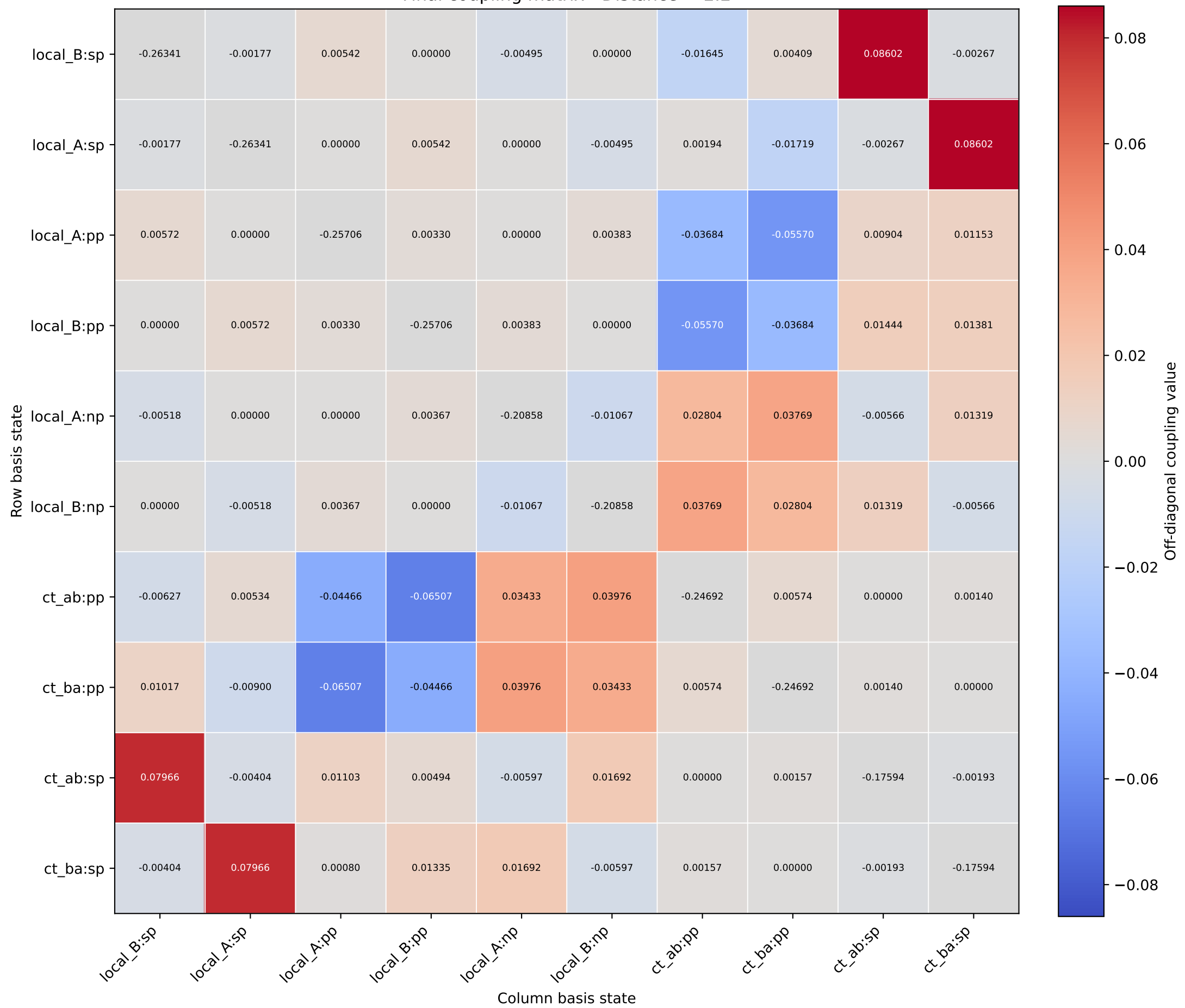
Final coupling matrix - Distance = 2.2
