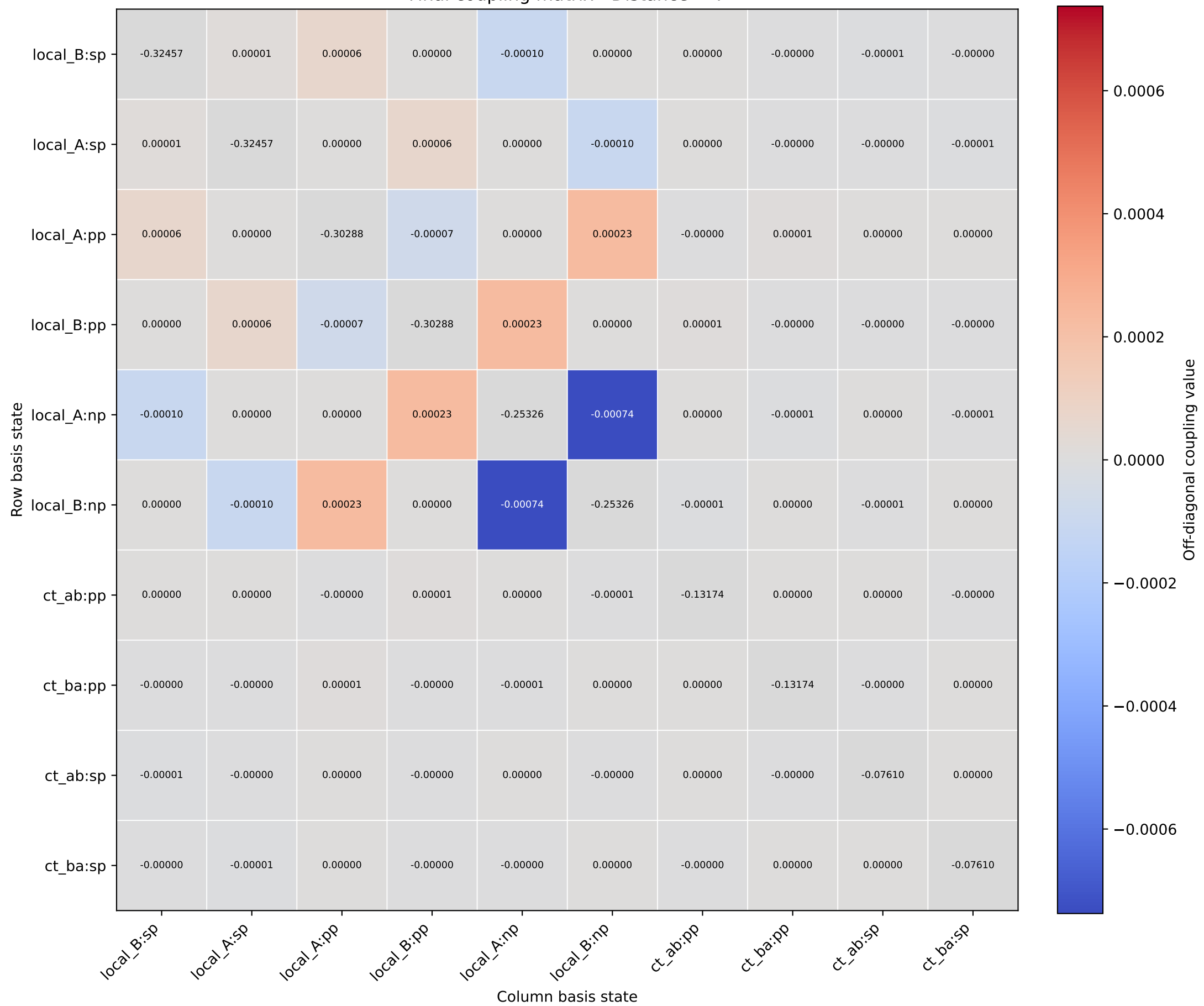
Final coupling matrix - Distance = 7
