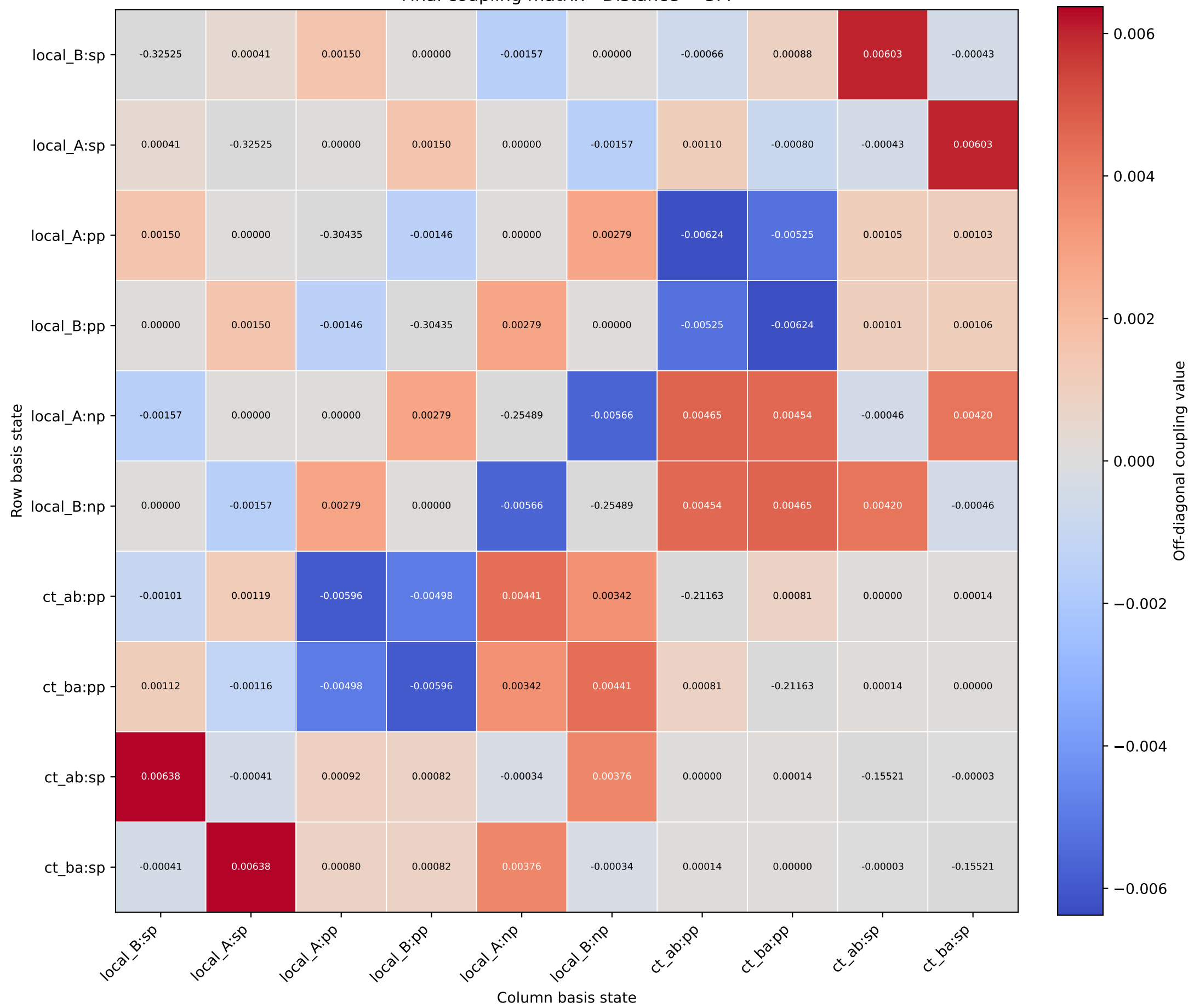
Final coupling matrix - Distance = 3.4
