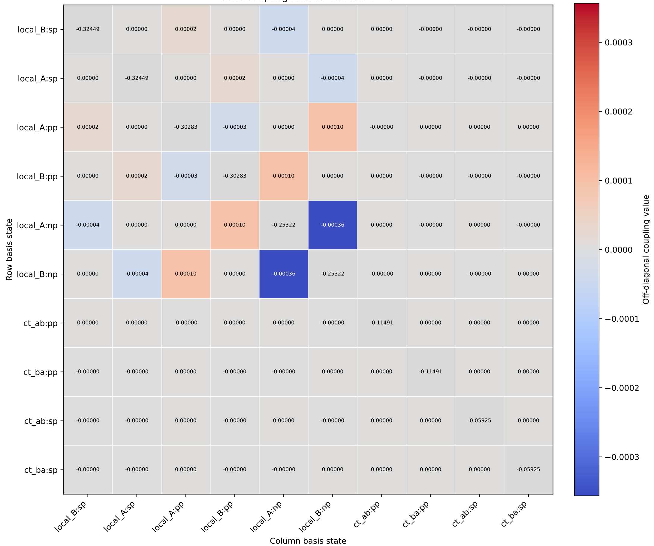
Final coupling matrix - Distance = 9
