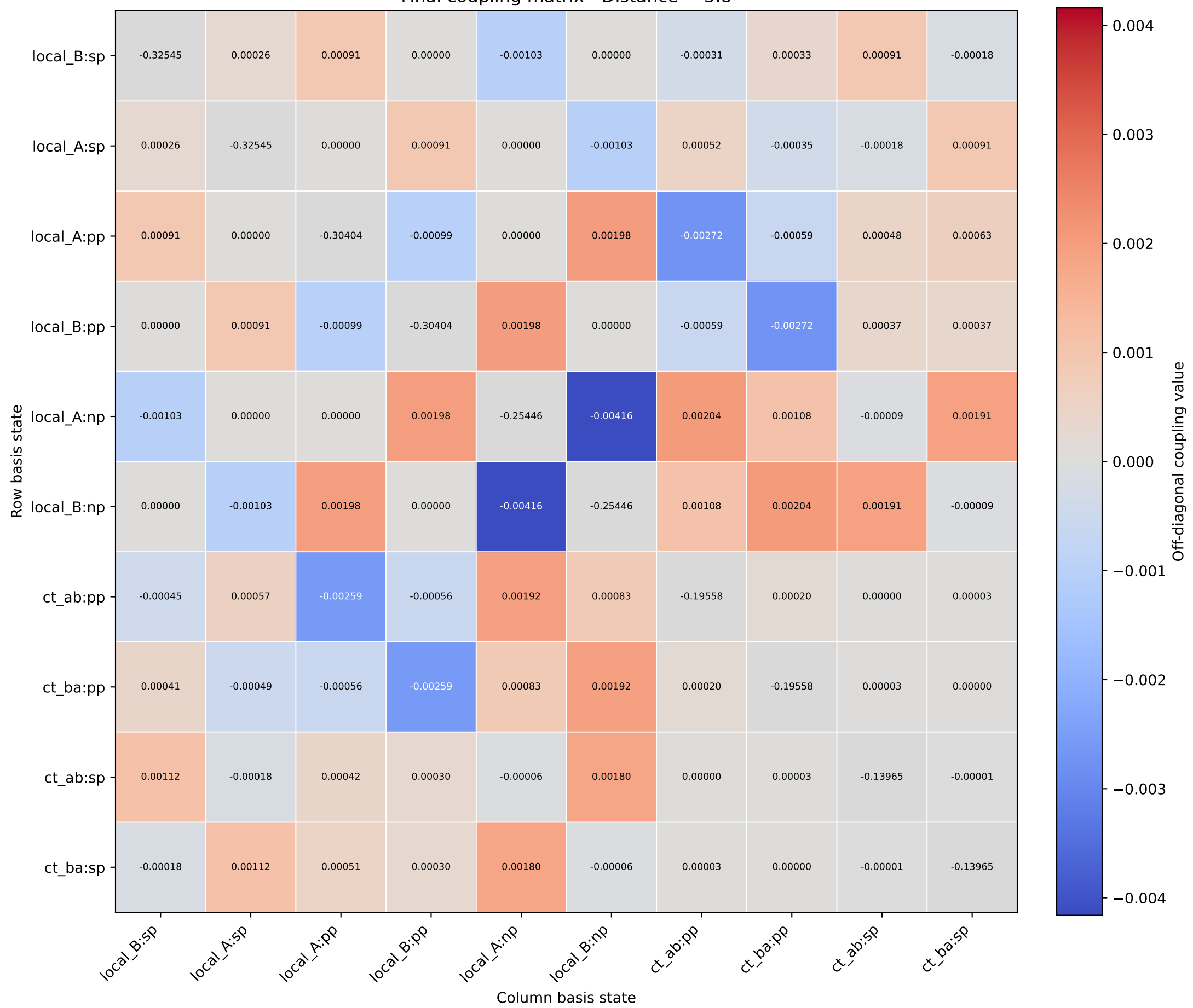
Final coupling matrix - Distance = 3.8
