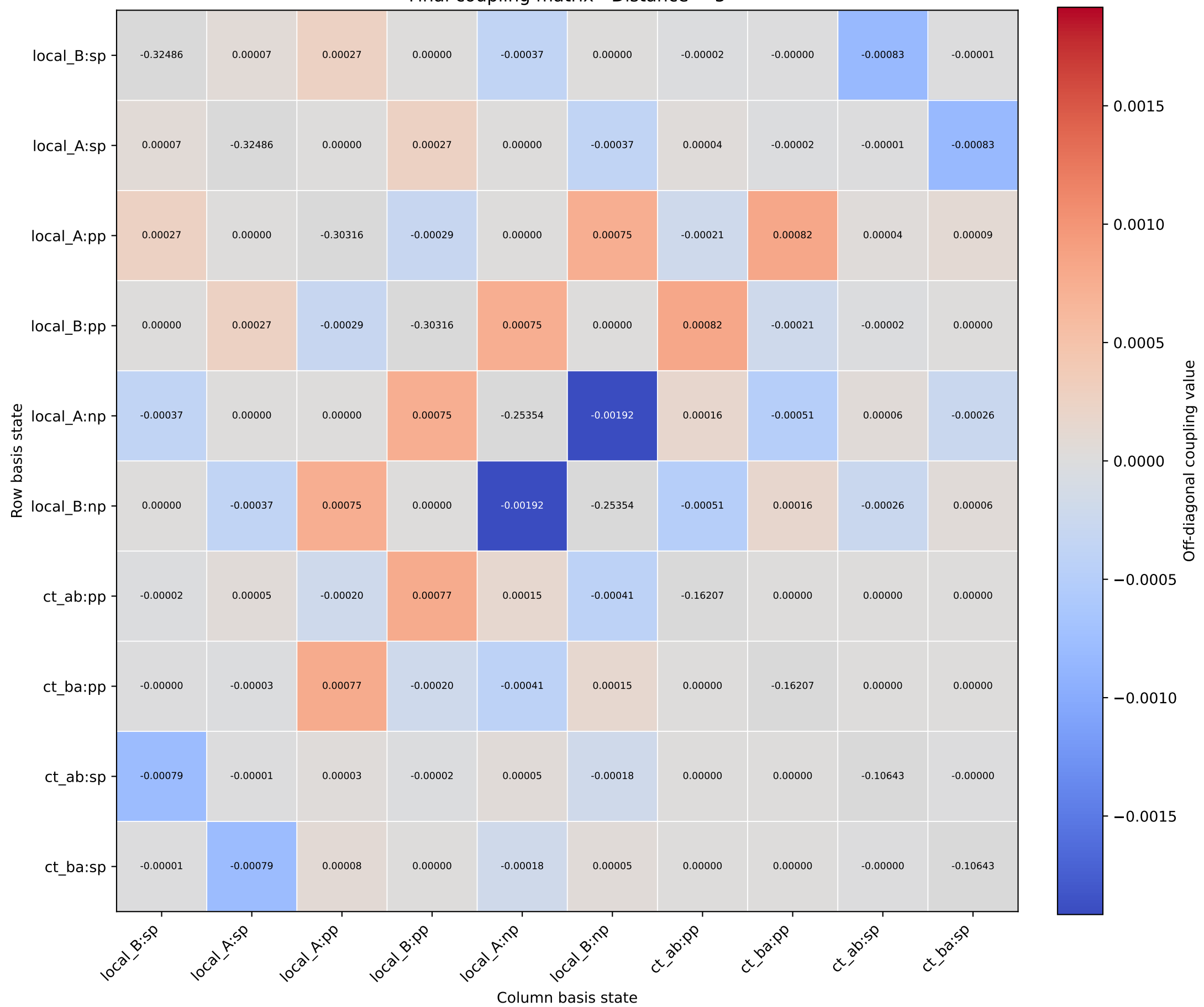
Final coupling matrix - Distance = 5
