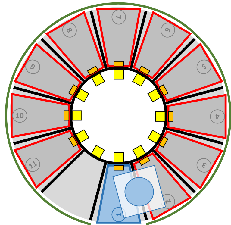
Step 2: if passed, position compartment no. 1 at disburse slot
