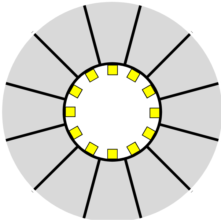
Inner vertical wall, side vertical wall, horizontal base, and magnets are part of the rotating component of the device
