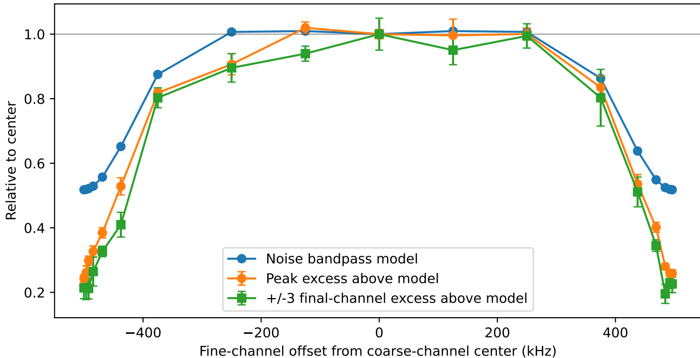
Noisy detected excess above modeled PFB bandpass
