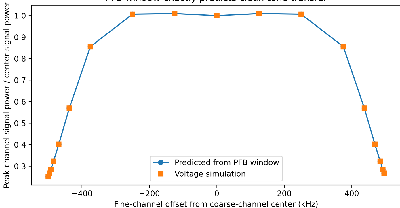
PFB window exactly predicts clean tone transfer
