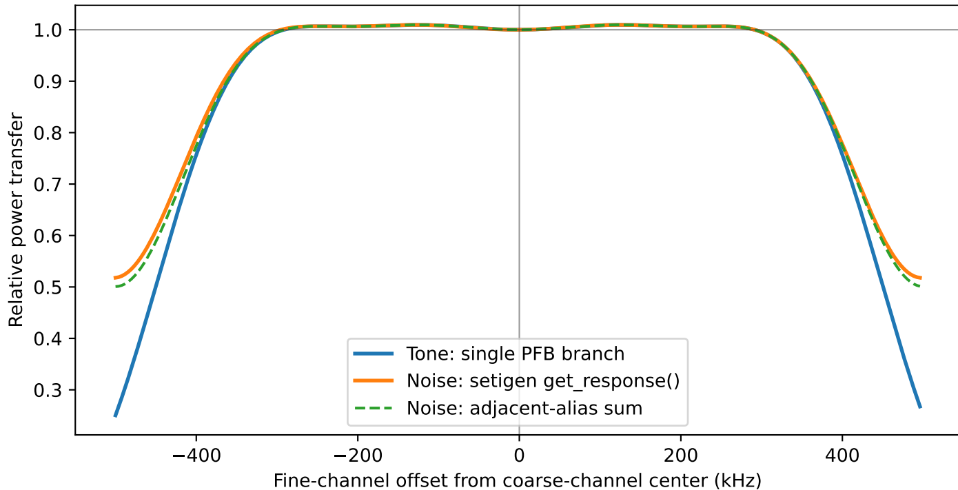
PFB tone transfer is not the same as the noise bandpass
