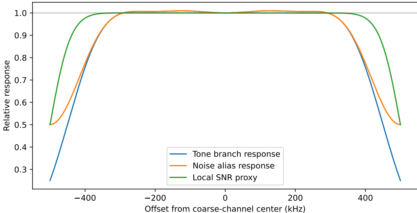
Analytic transfer functions from the PFB prototype
